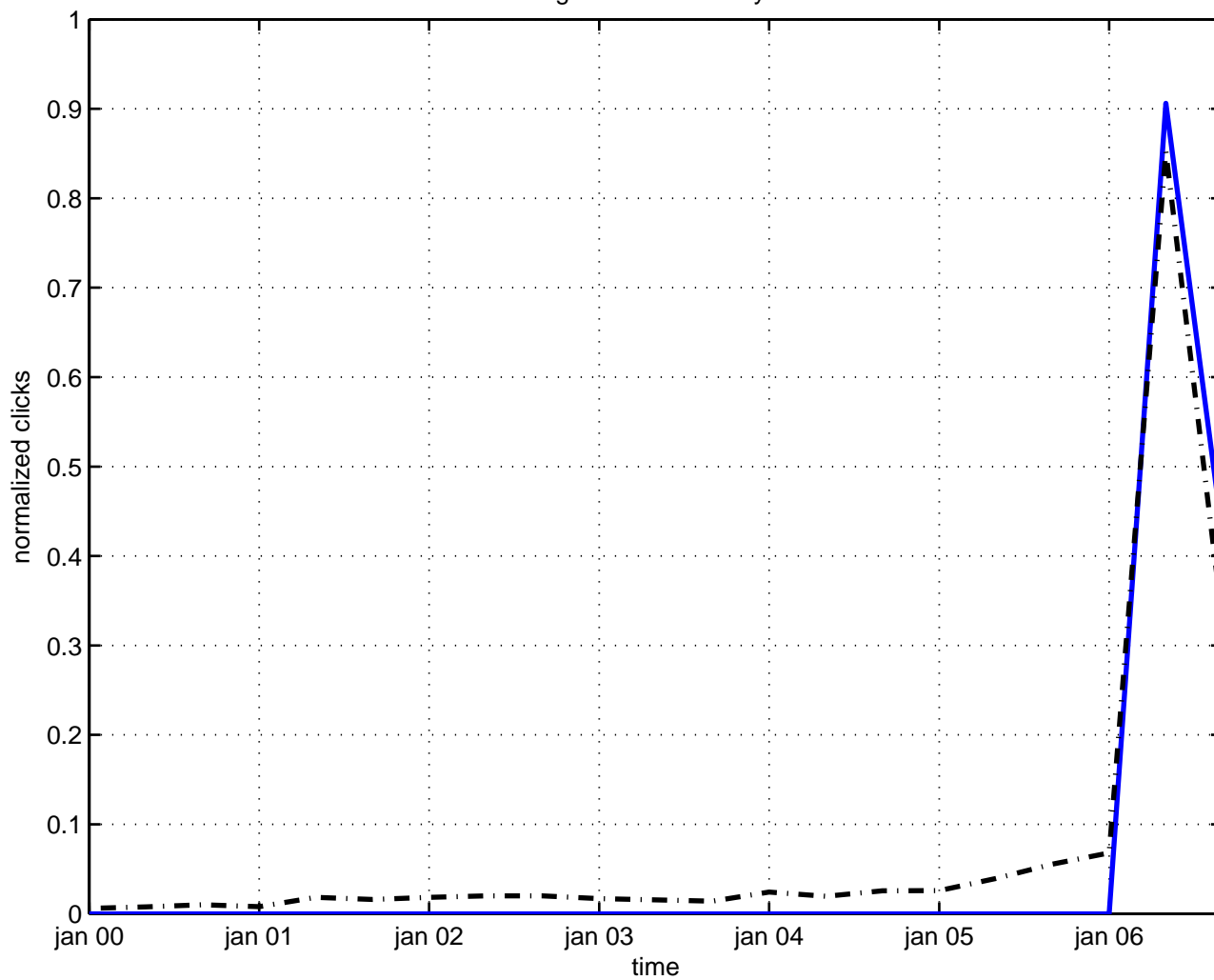
light cone m-theory
