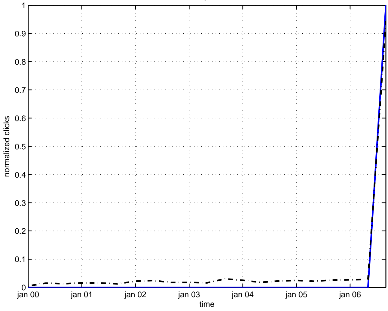
lifetime space-time
