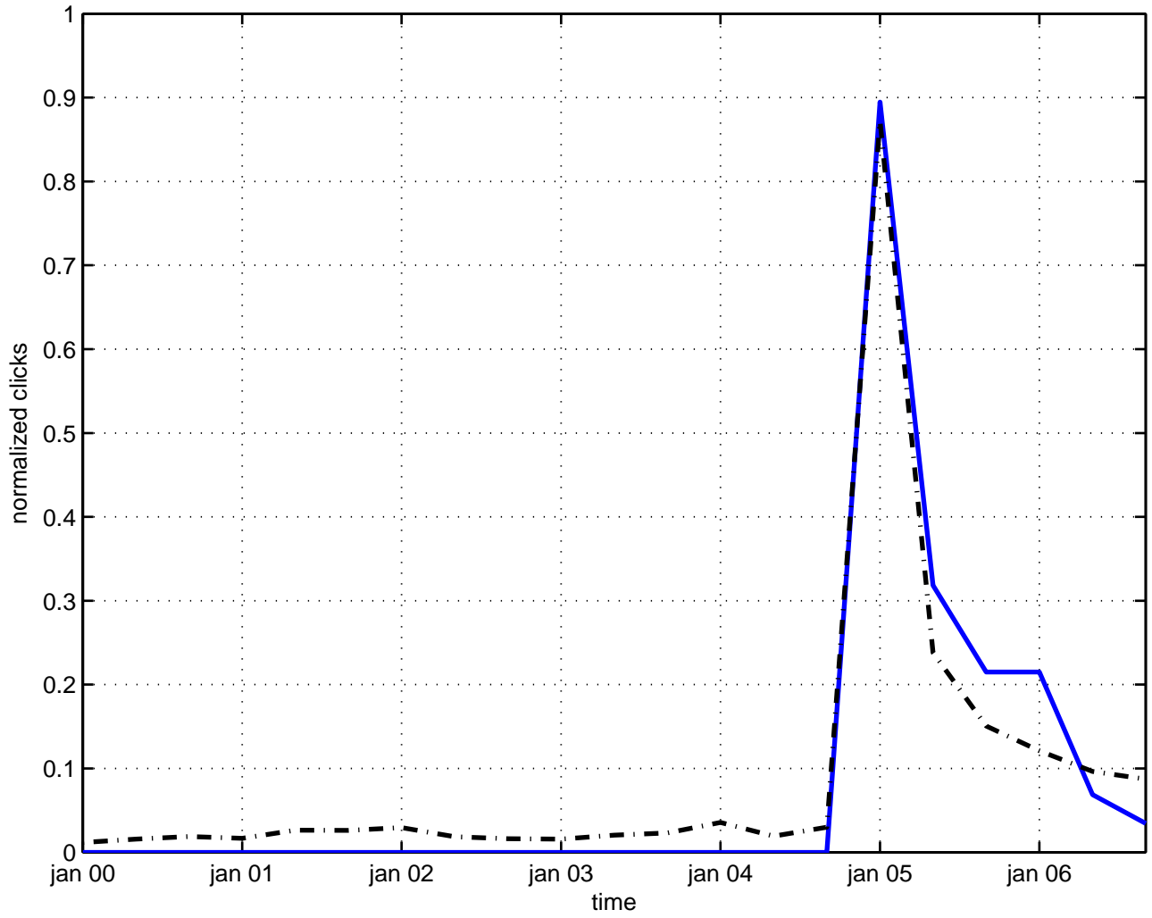
lifetime soliton
