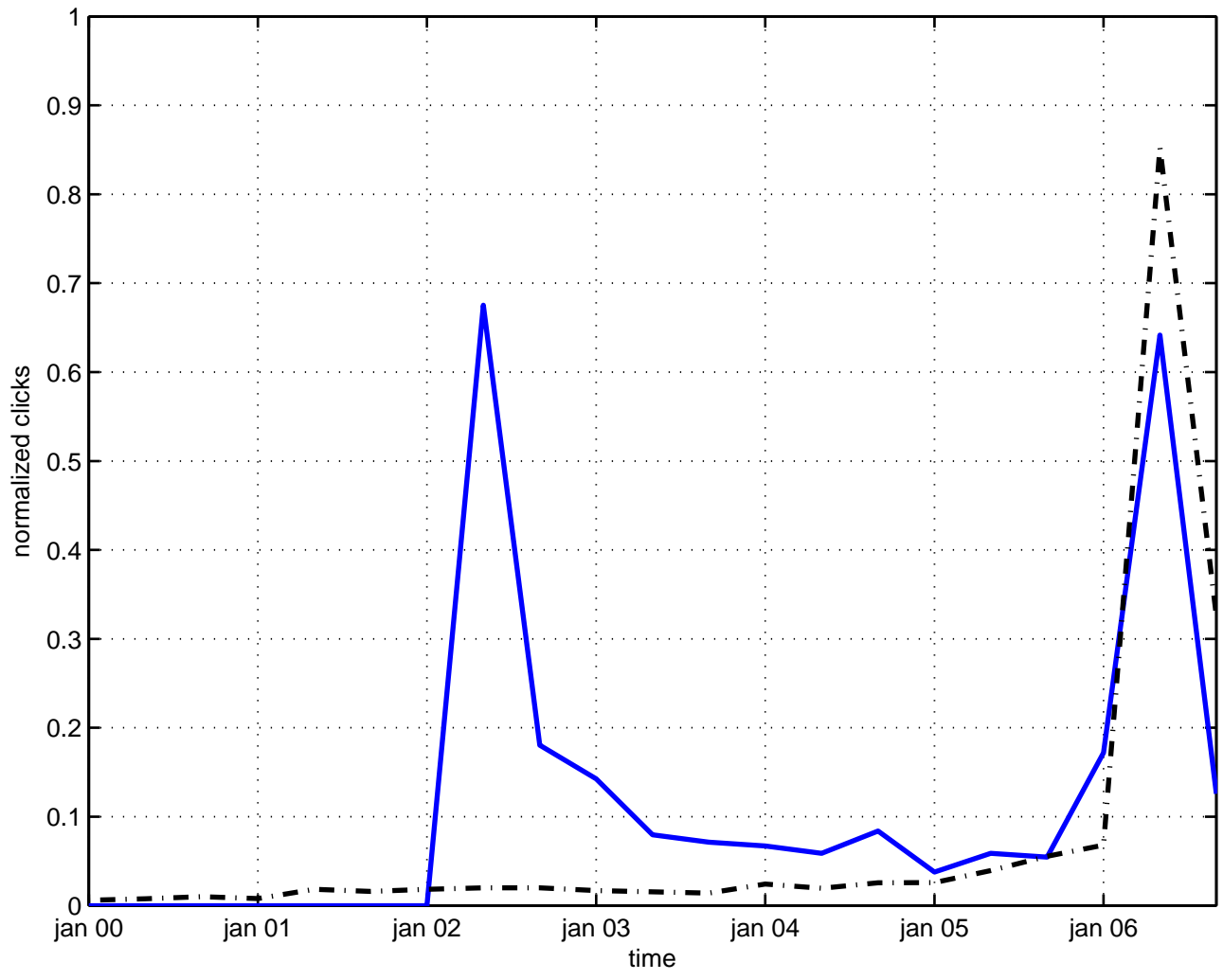
lie derivative
