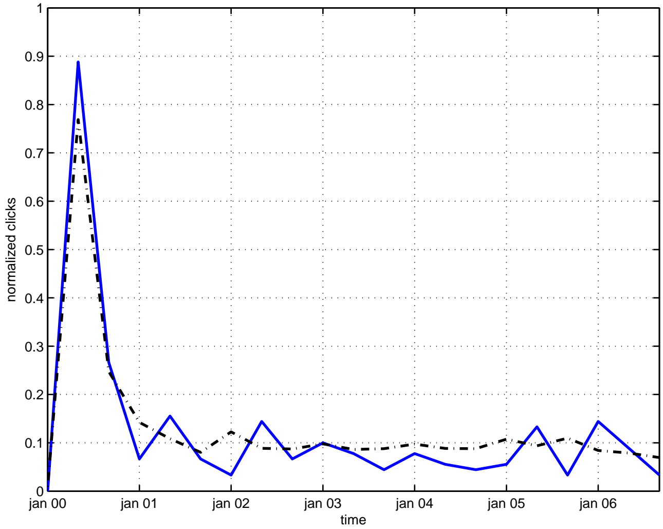
lee-yang singularity
