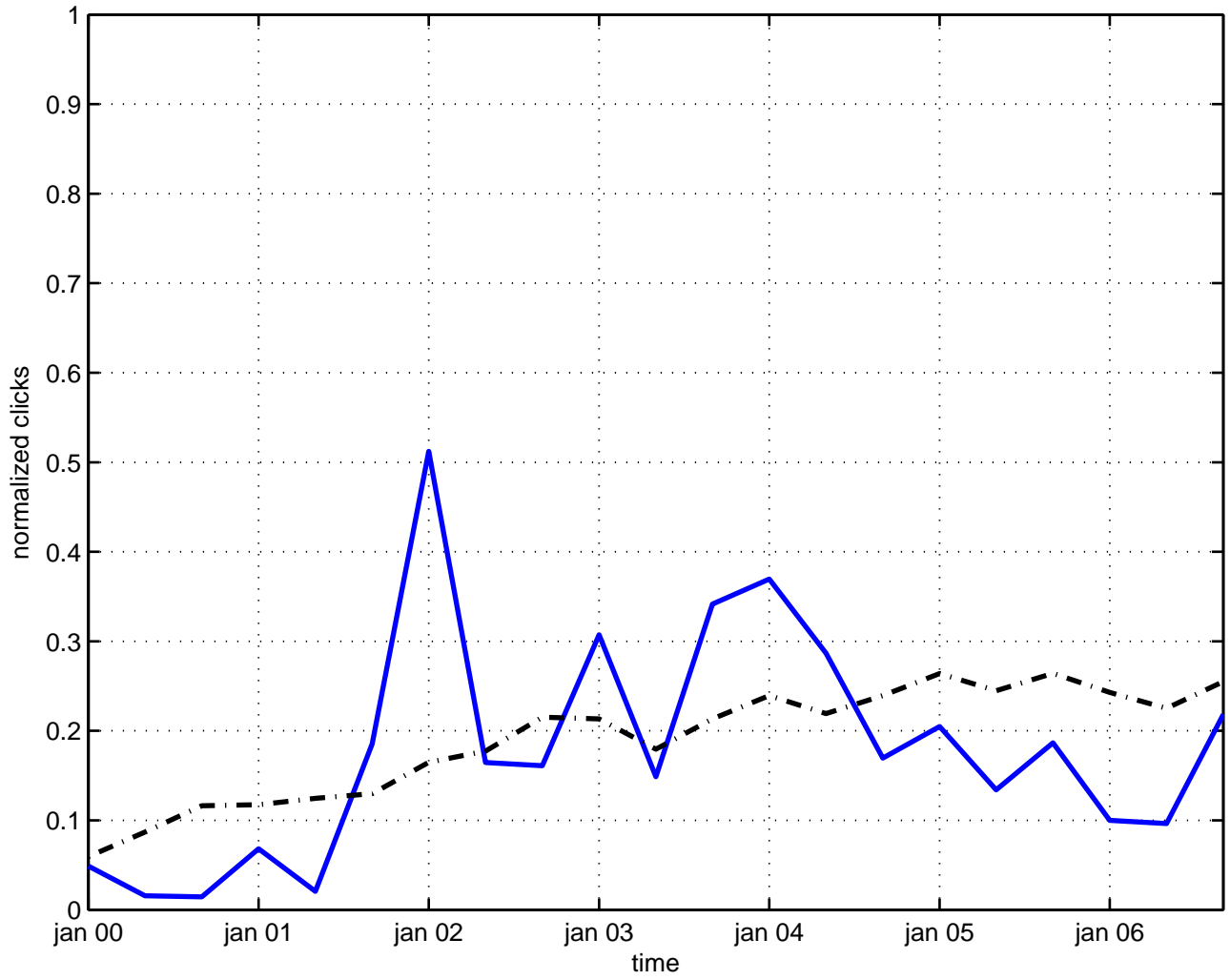
lax pair
