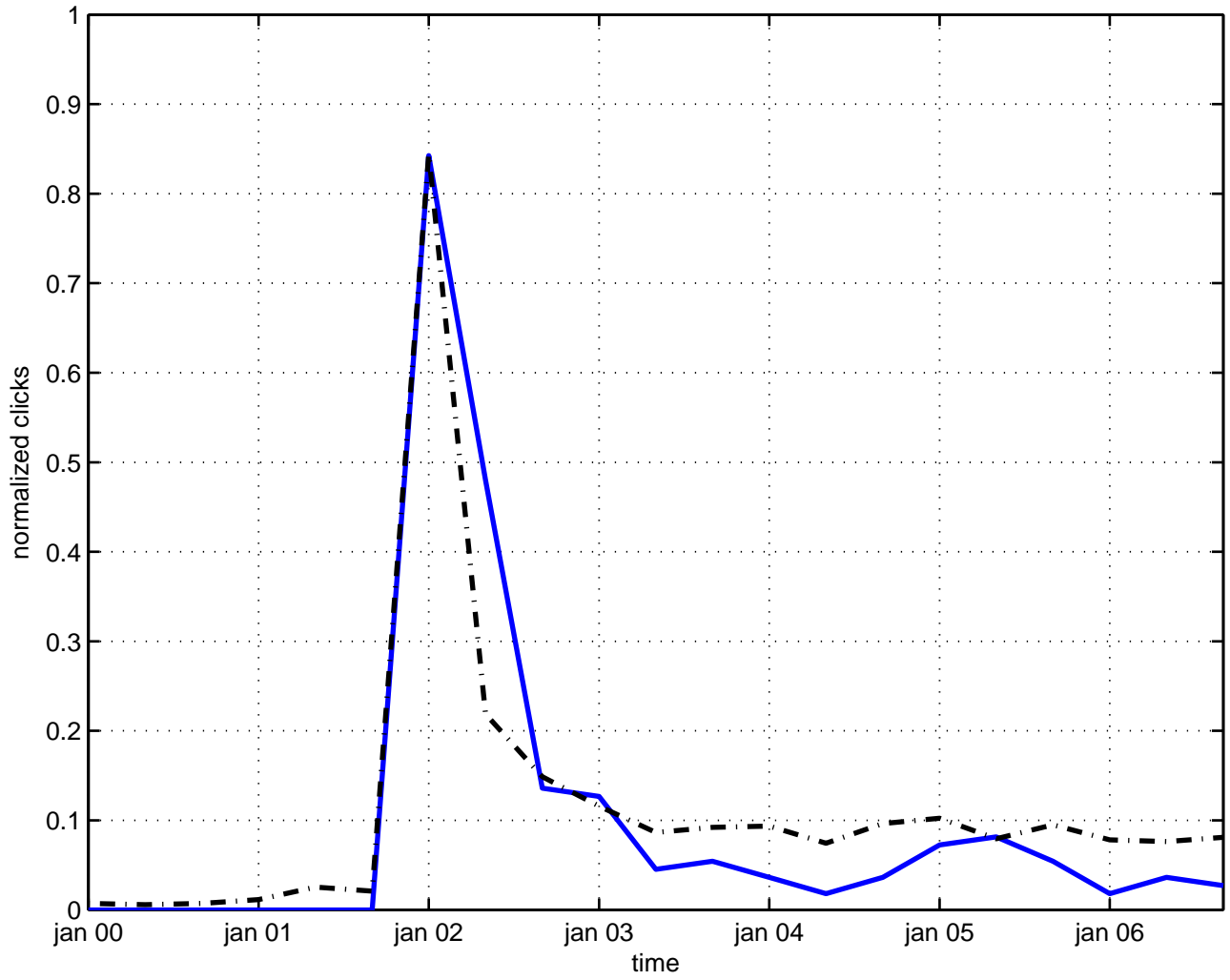
lattice operator
