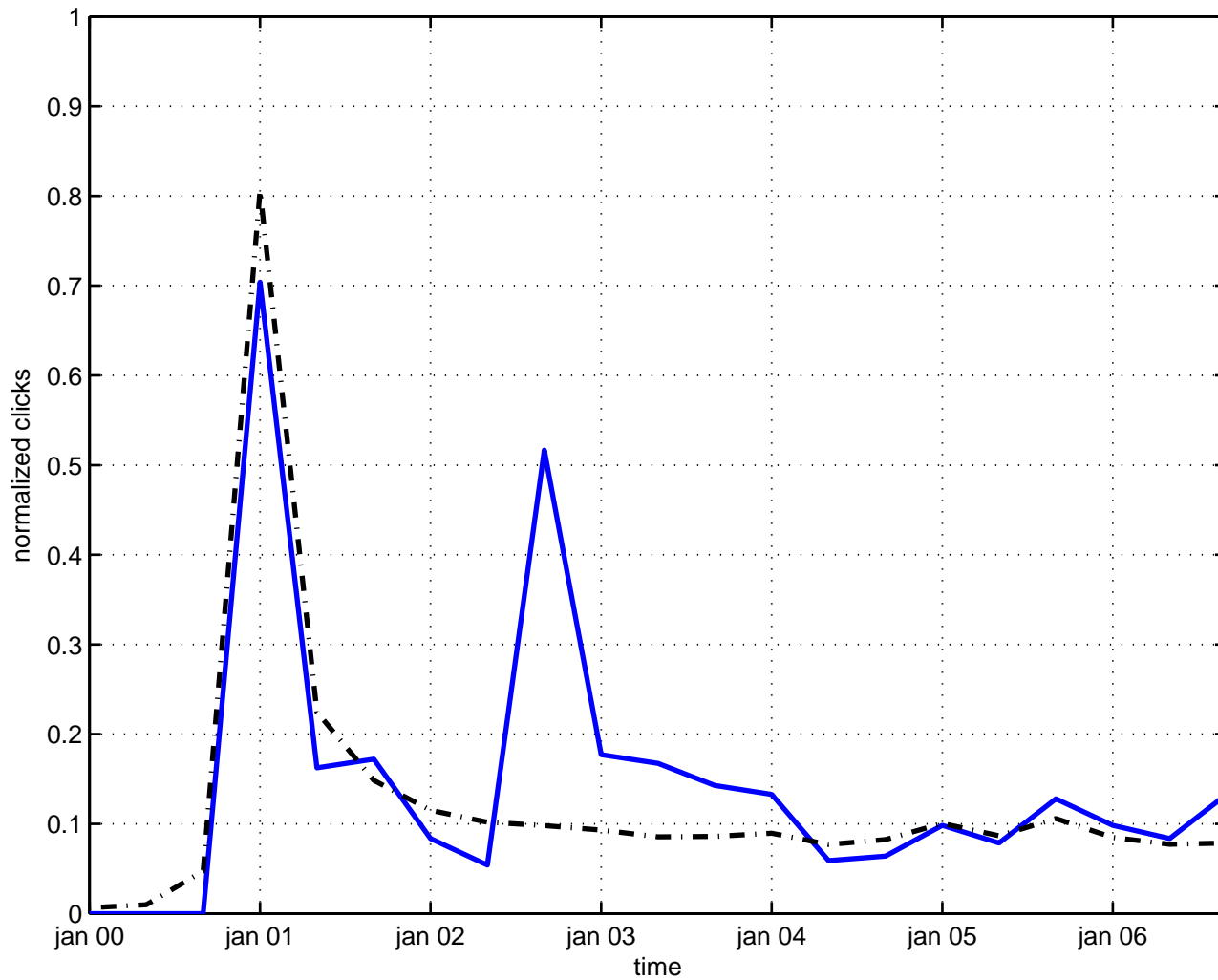
lattice model
