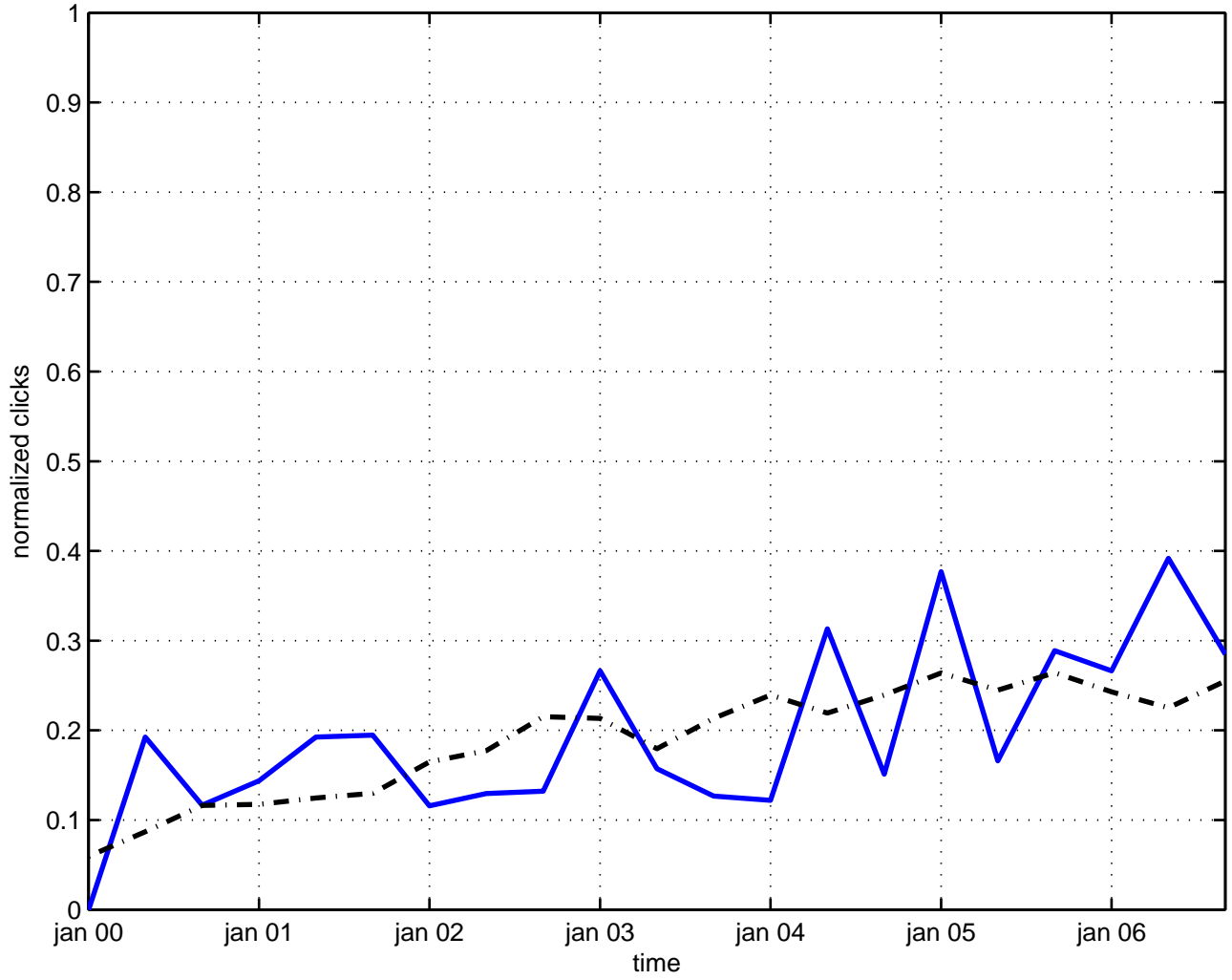
langevin equation
