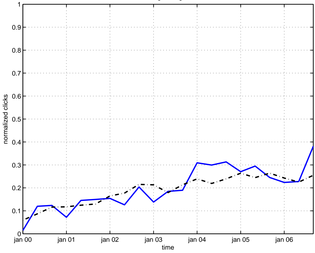
landau-ginzburg model
