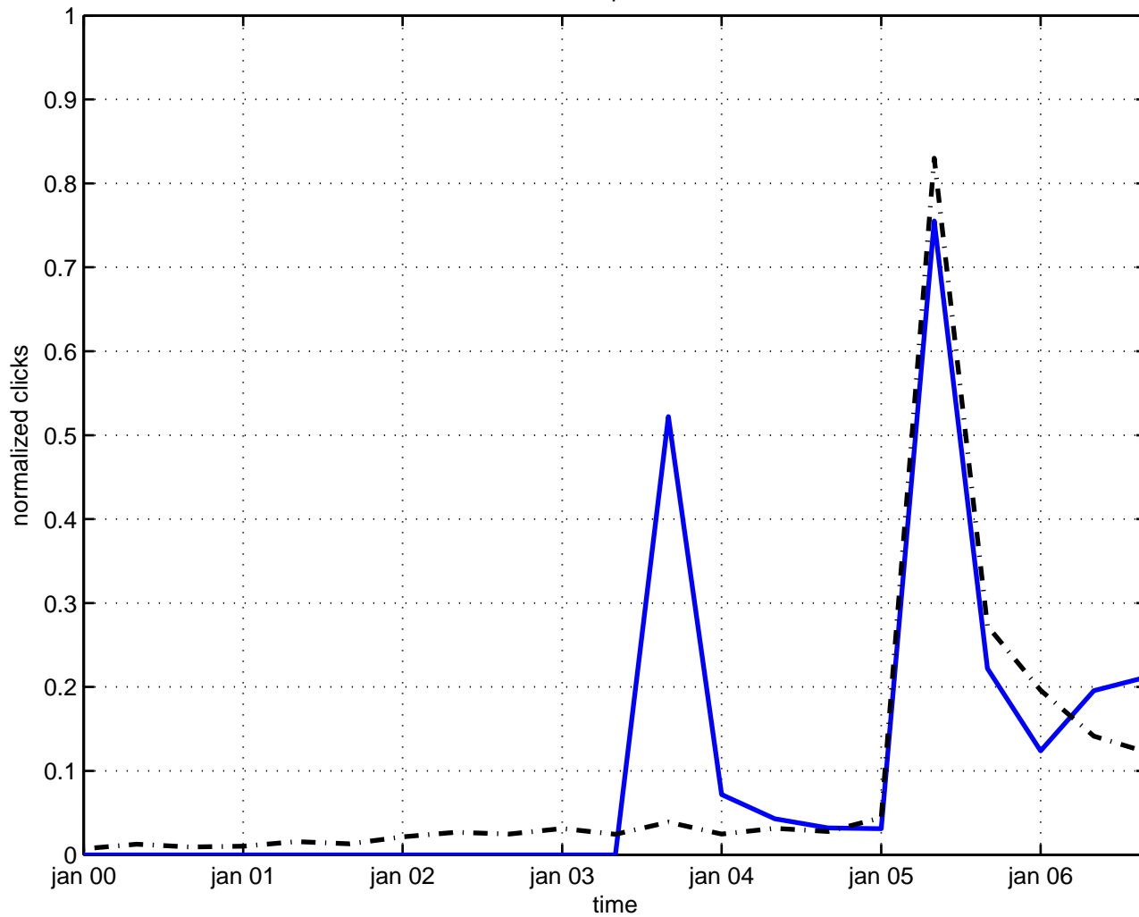
landau problem
