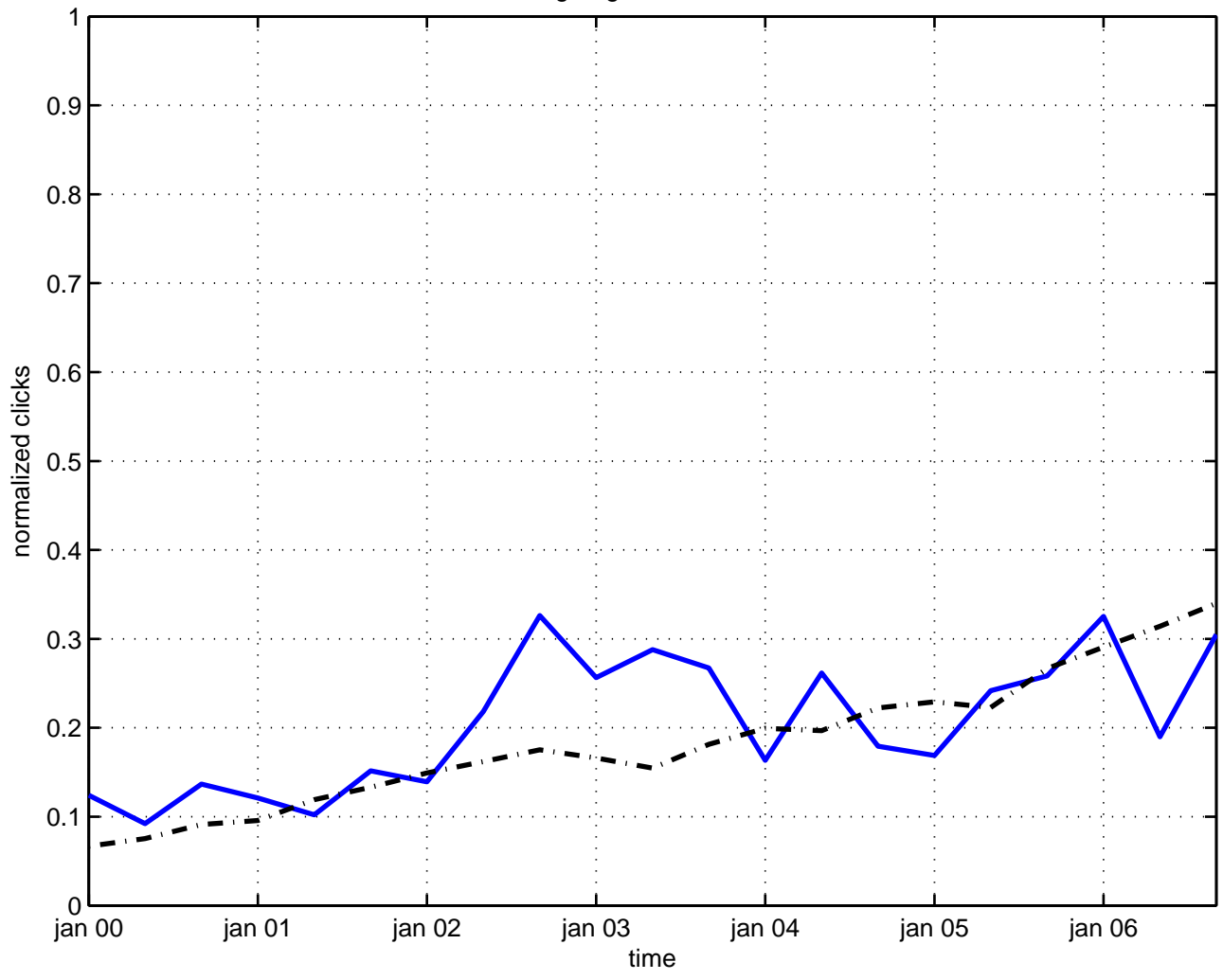
lagrangian formalism
