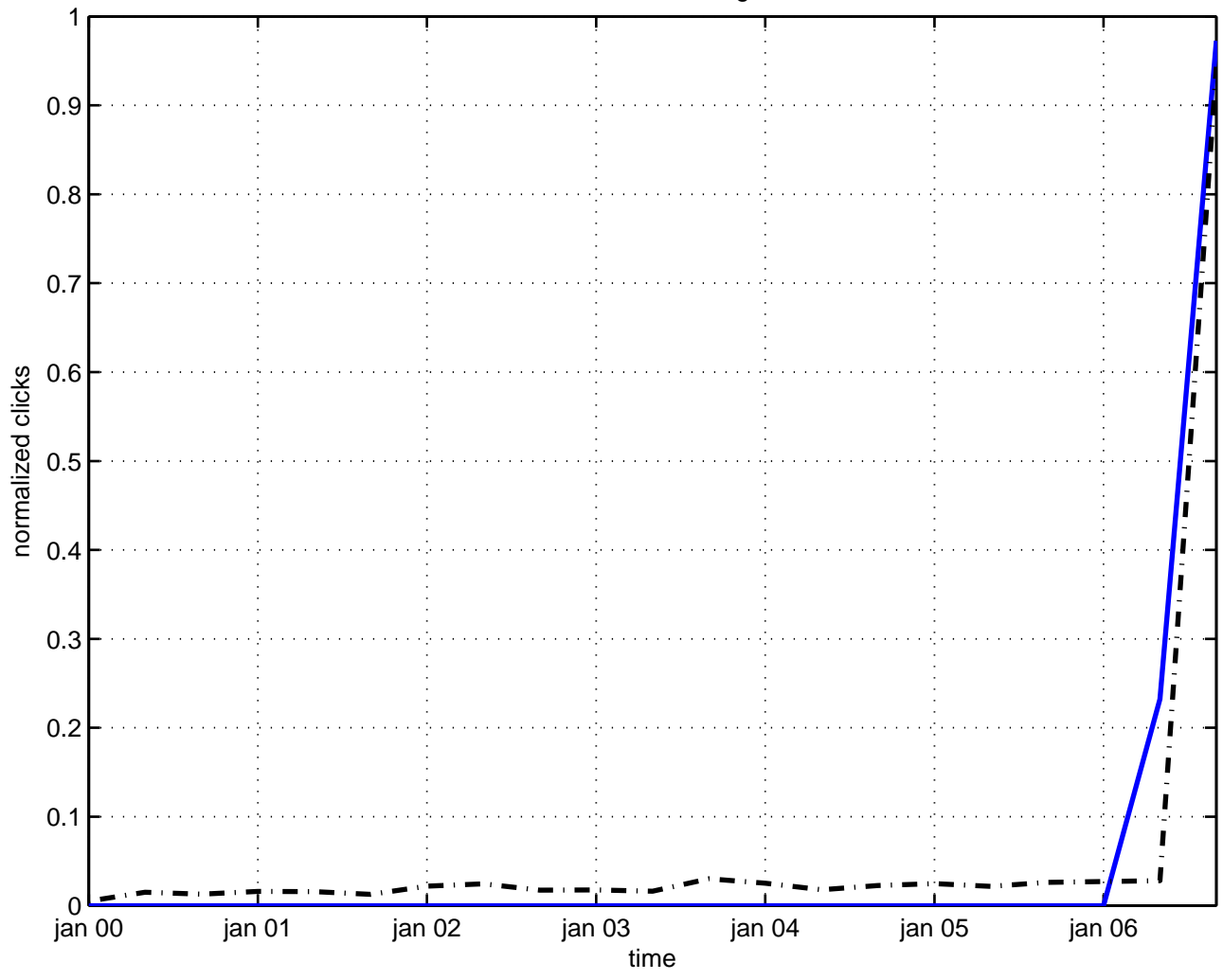
krichever–novikov algebra
