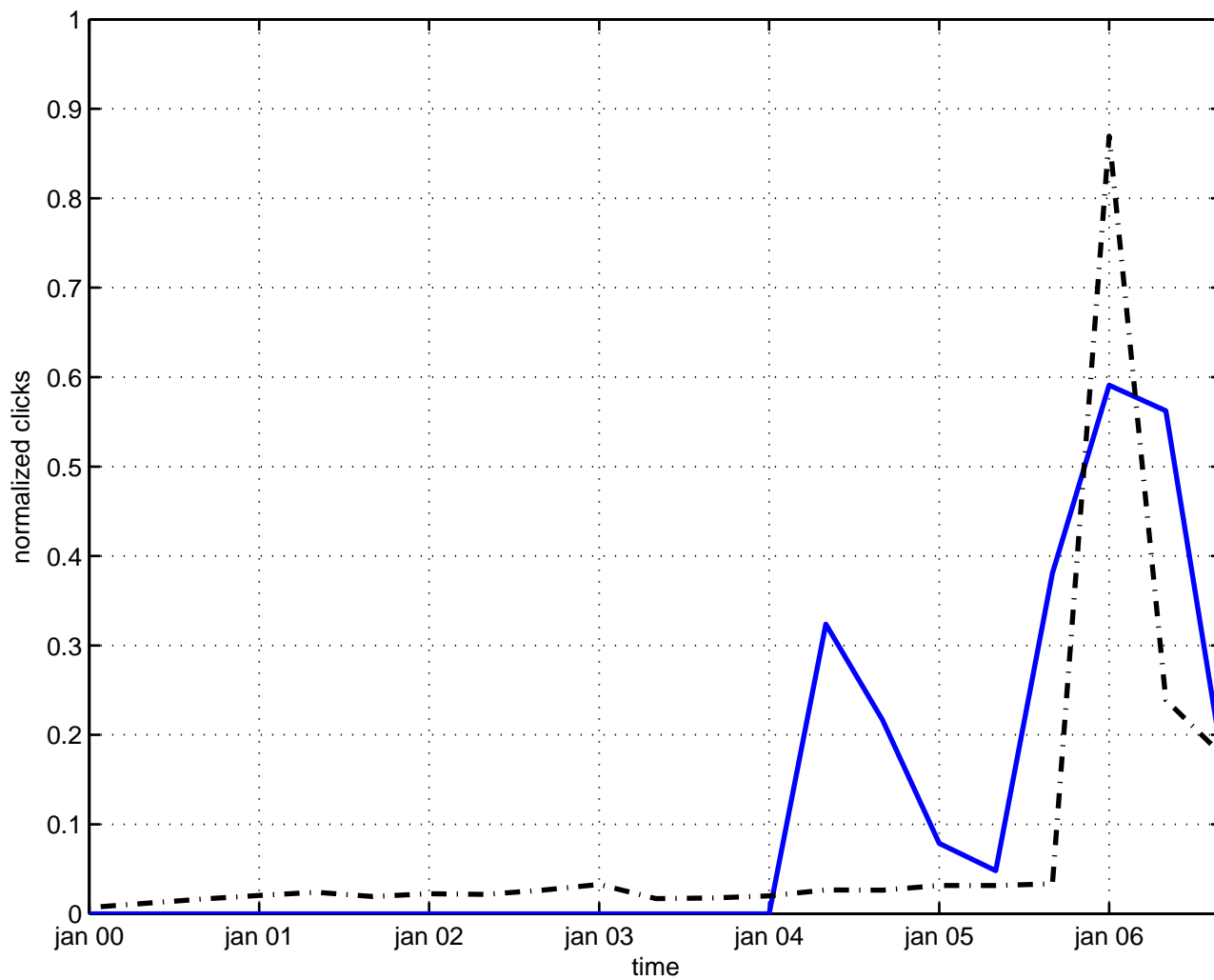
kontsevich model
