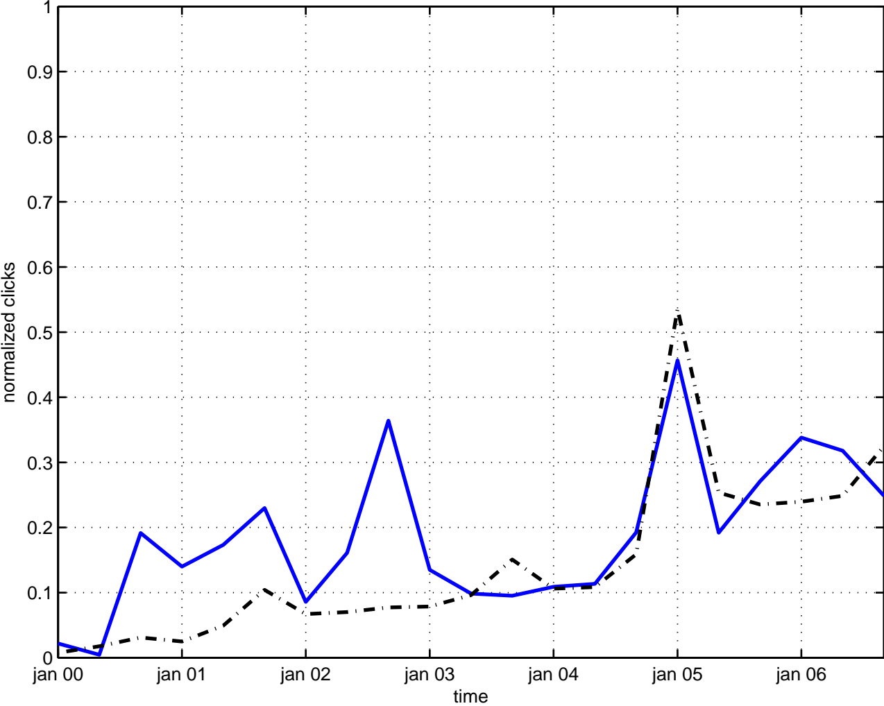
knizhnik-zamolodchikov equation
