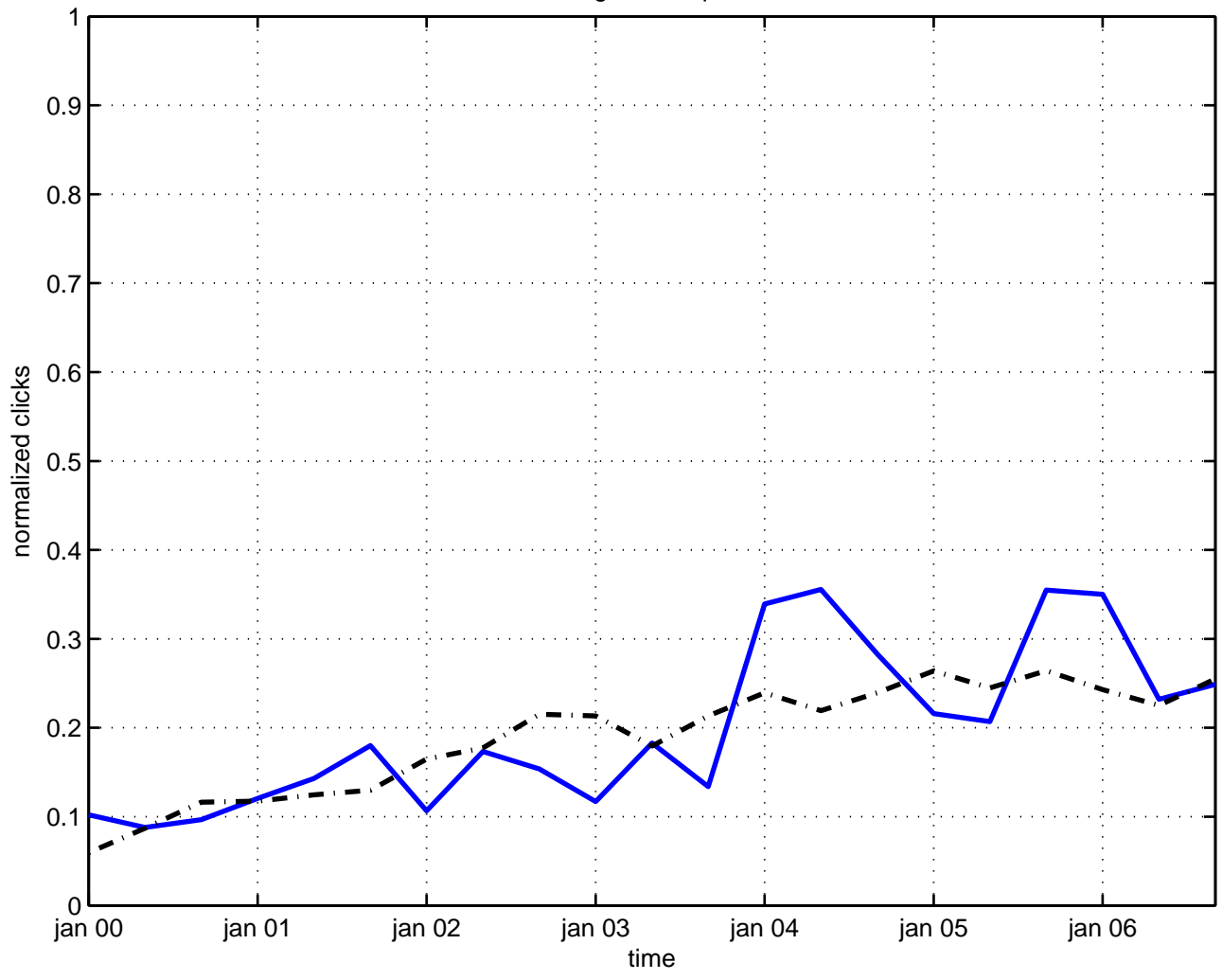
klein-gordon equation
