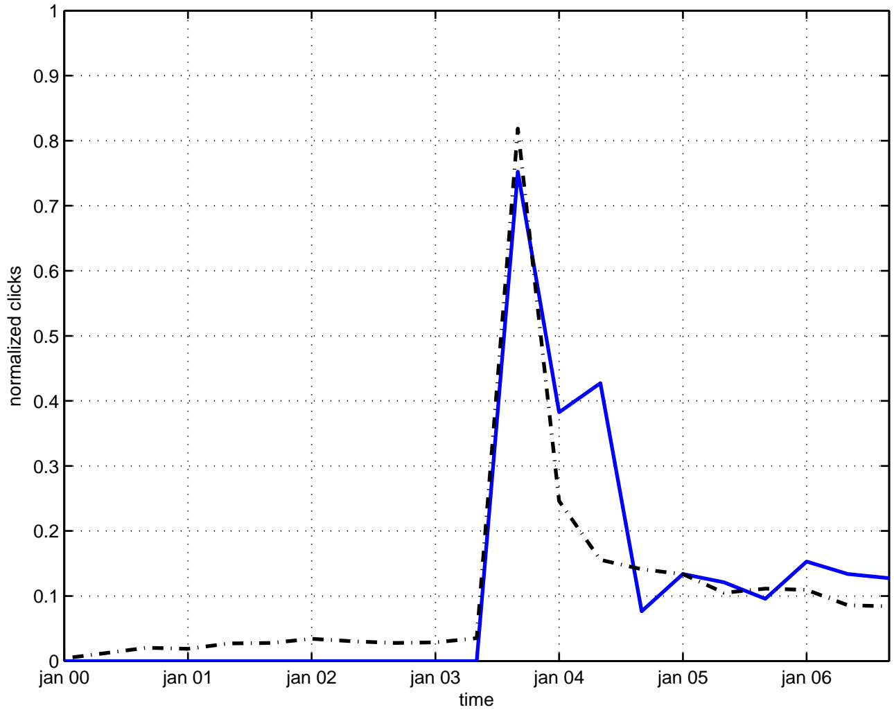
klein paradox
