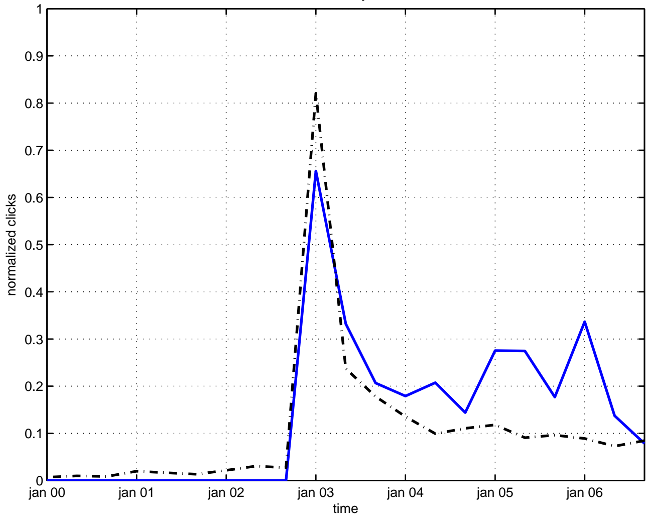
kink tachyon
