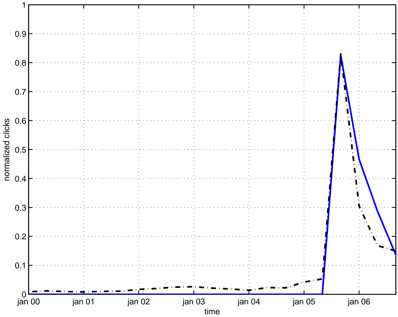
kinetics energy
