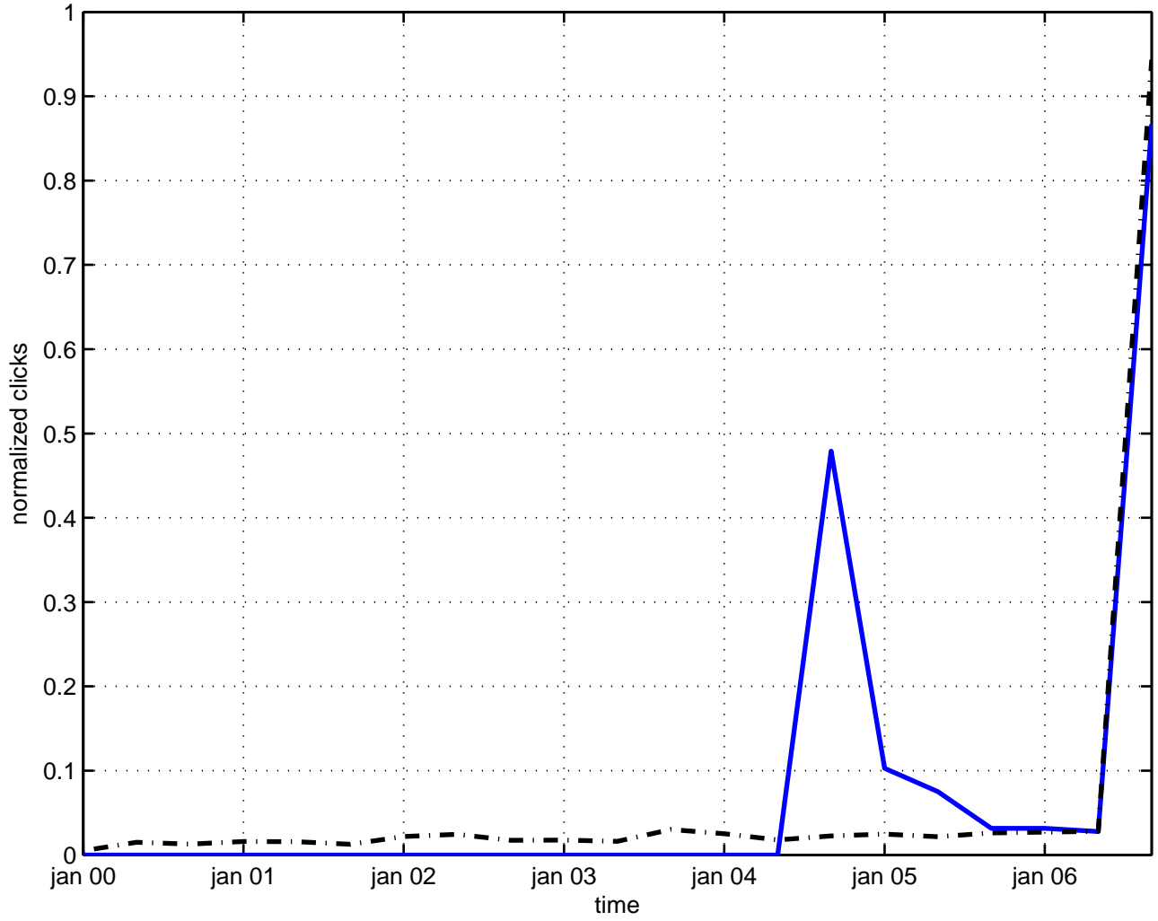
killing-yano tensor
