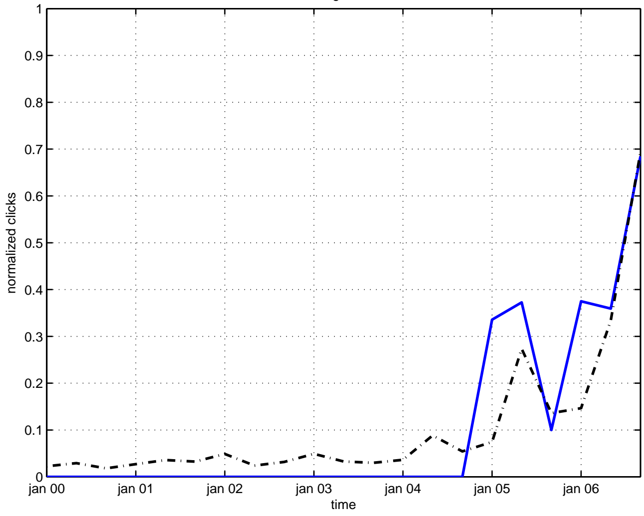
killing tensor
