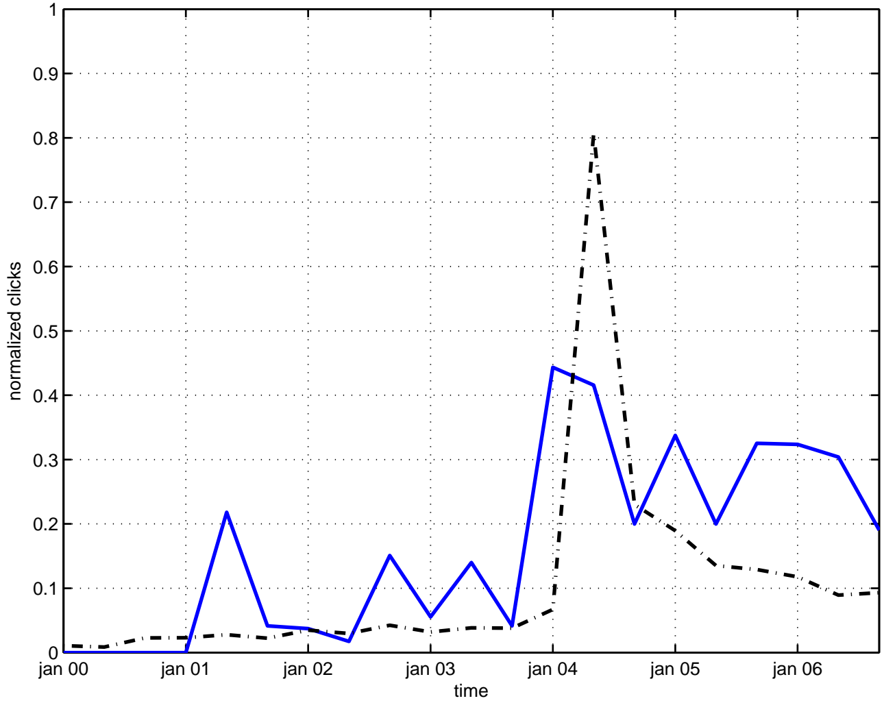
killing horizon
