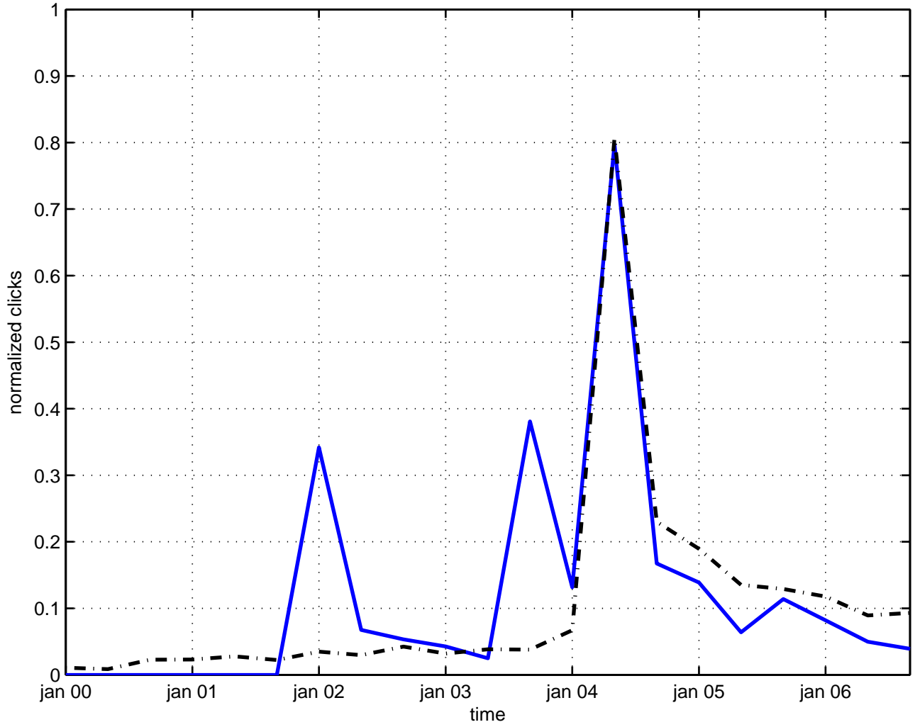
killing differential equations
