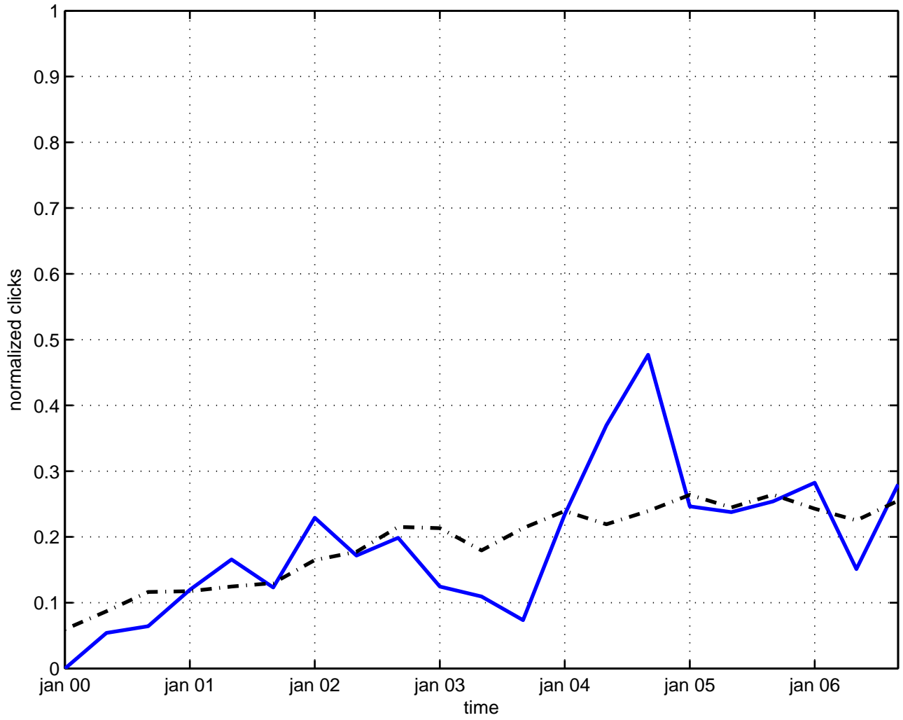
kerr space-time
