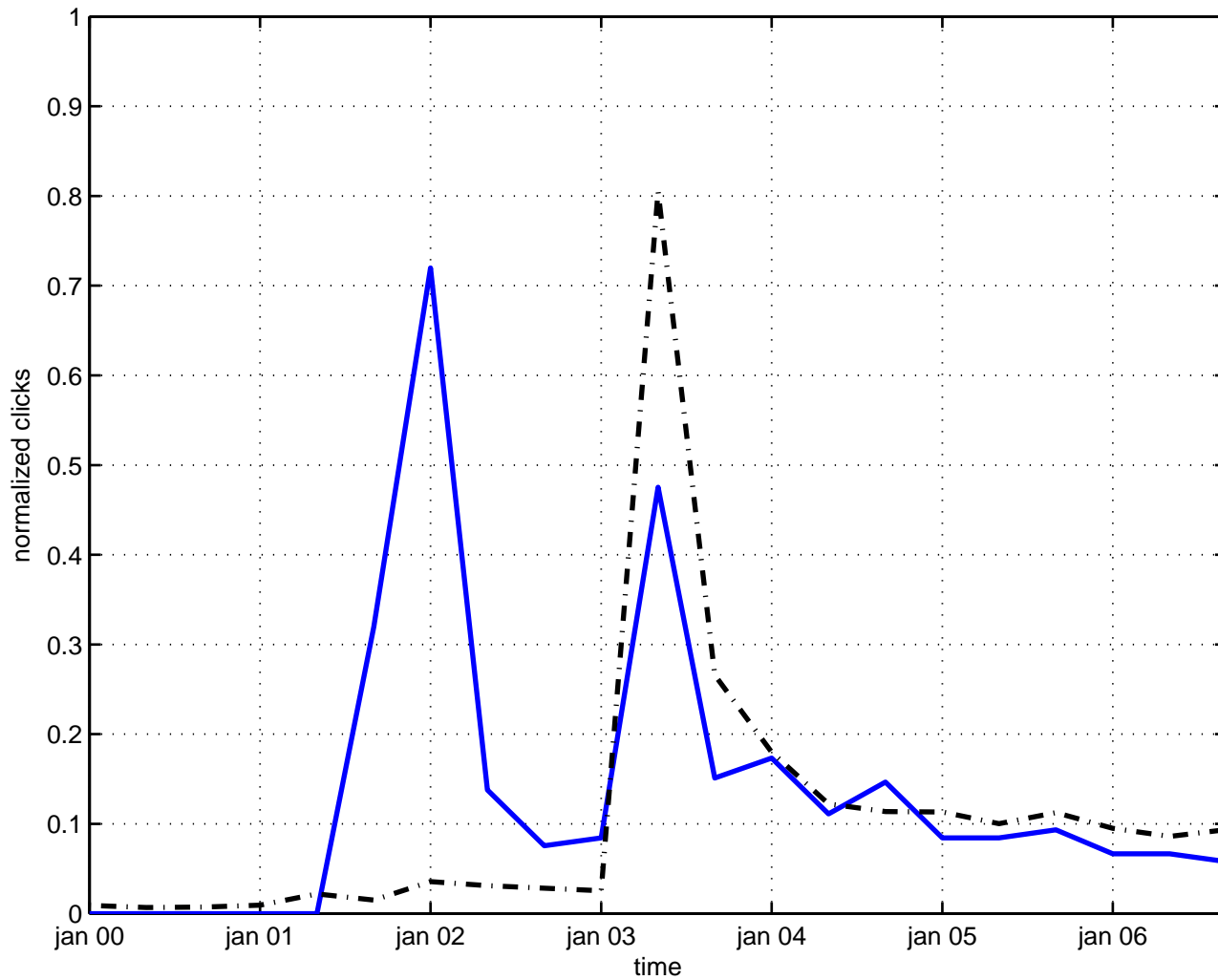
kazama-suzuki model
