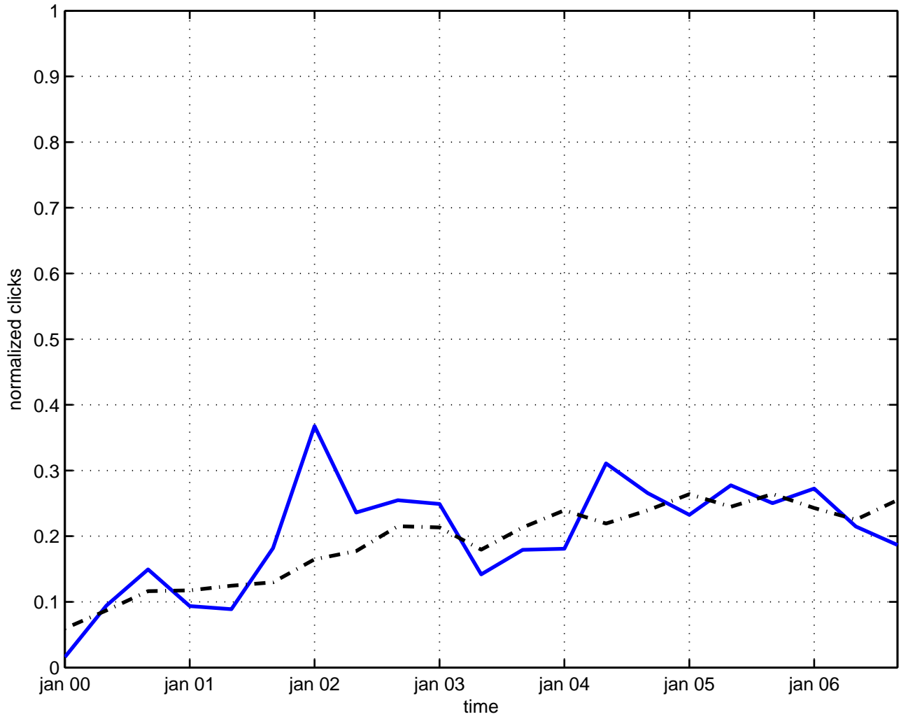
kappa symmetry
