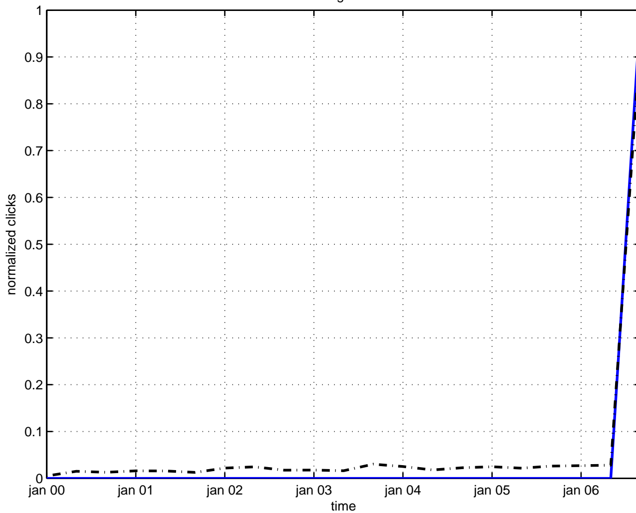
kaehler gravitation
