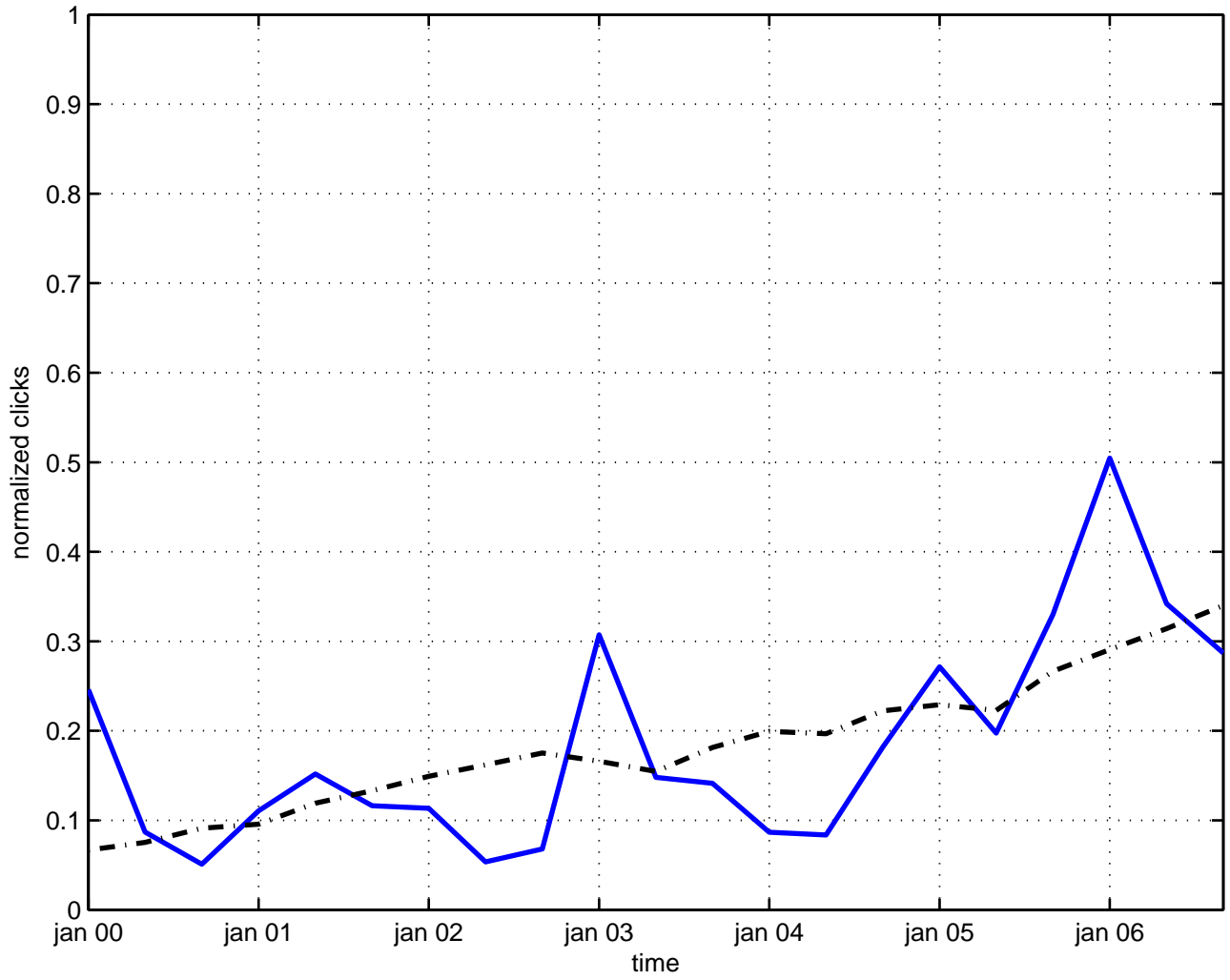
kaehler geometry
