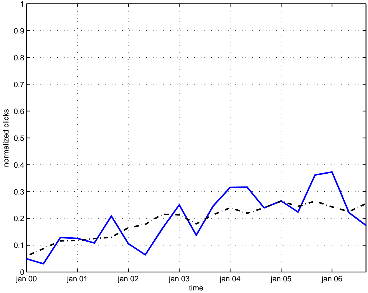
kaehler field theory
