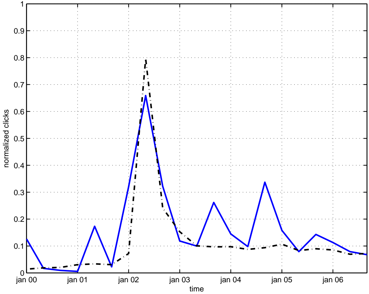
kaehler coset space
