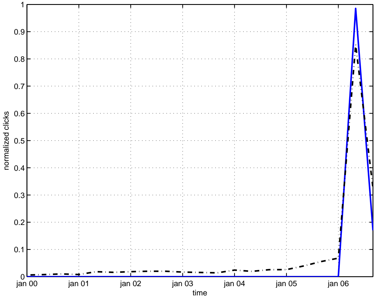
kaehler anomaly
