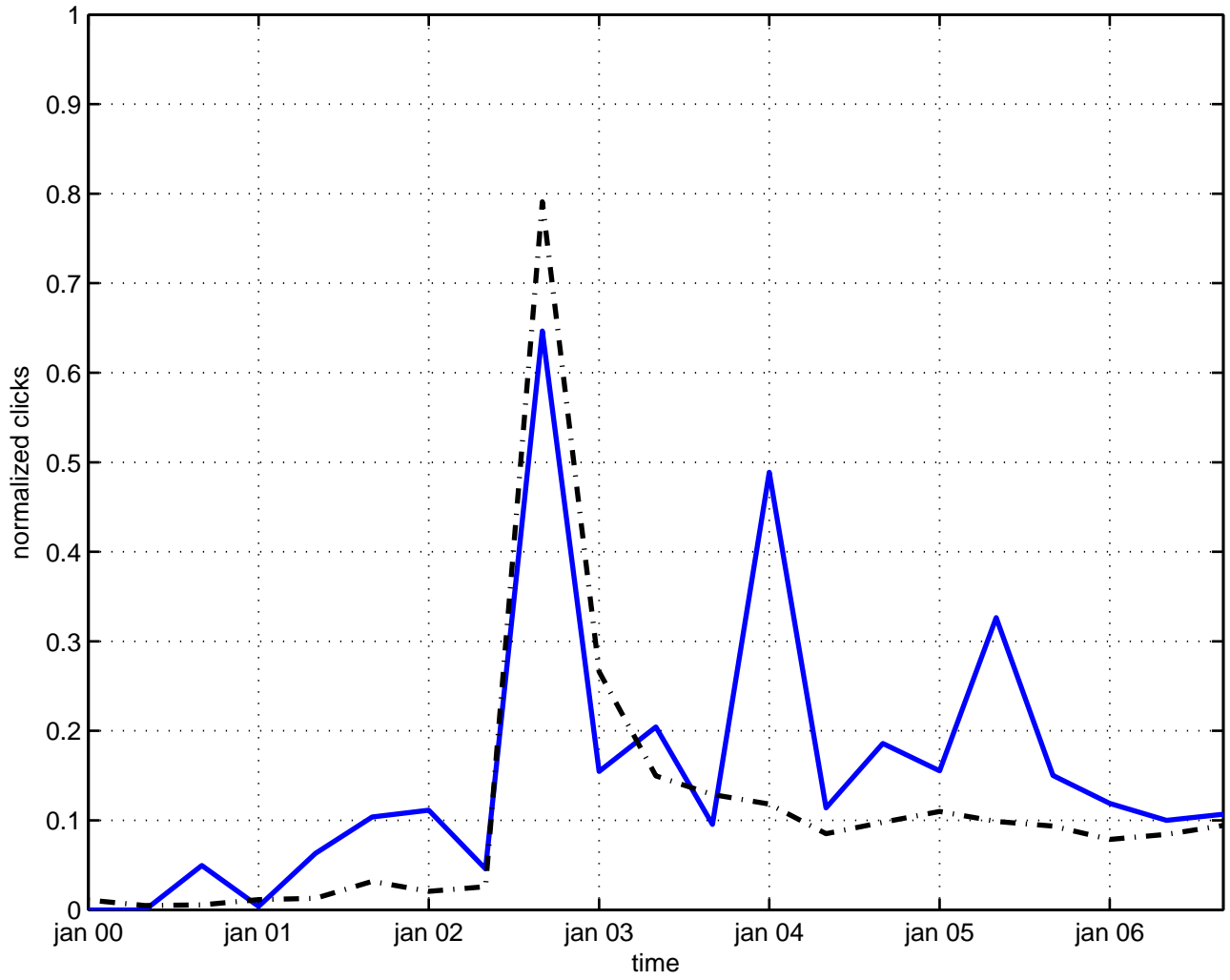
kadomtsev-petviashvili equation
