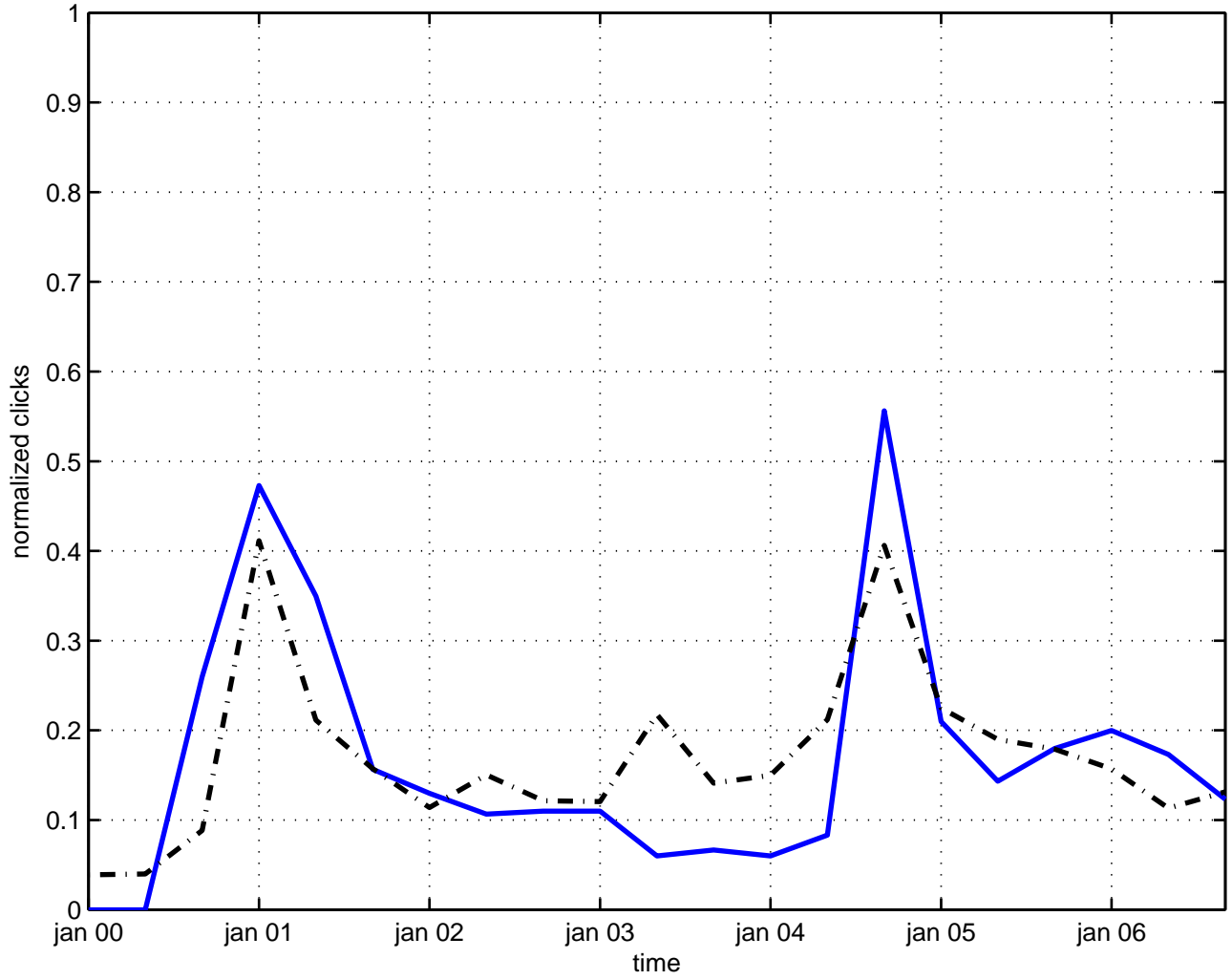
kac-moody group theory
