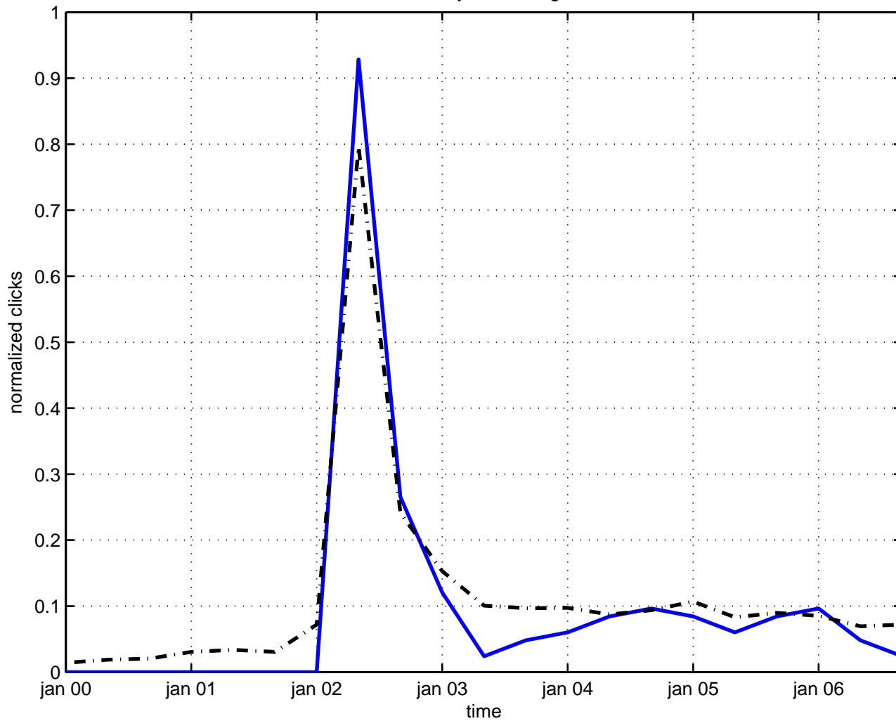
kac-moody current algebra
