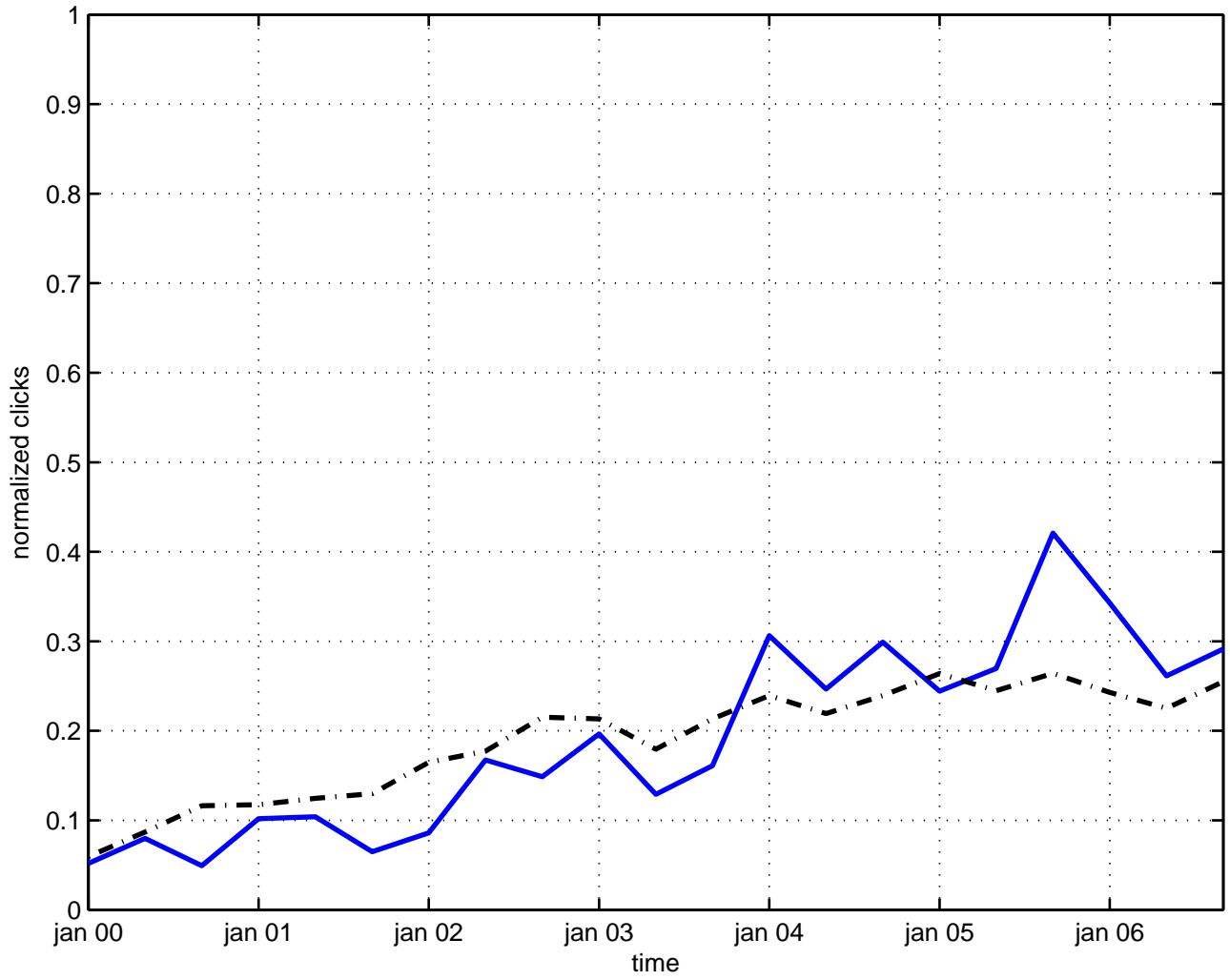
kac-moody algebra
