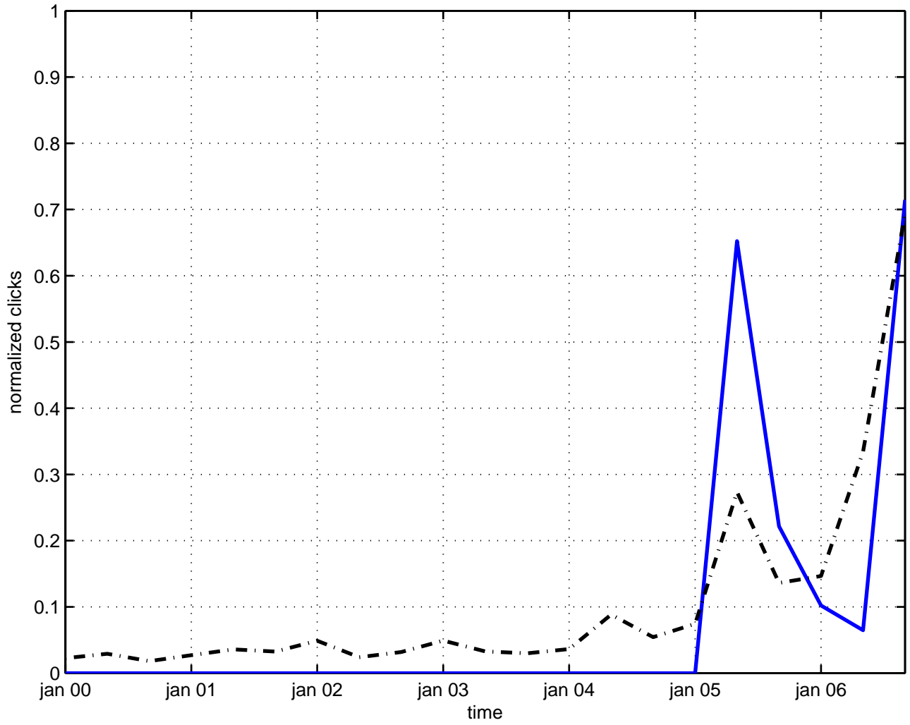
k(3) x t(2) space
