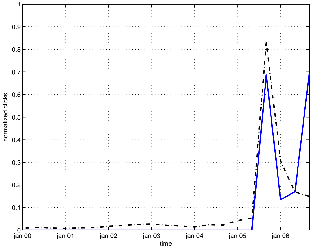
josephson effect
