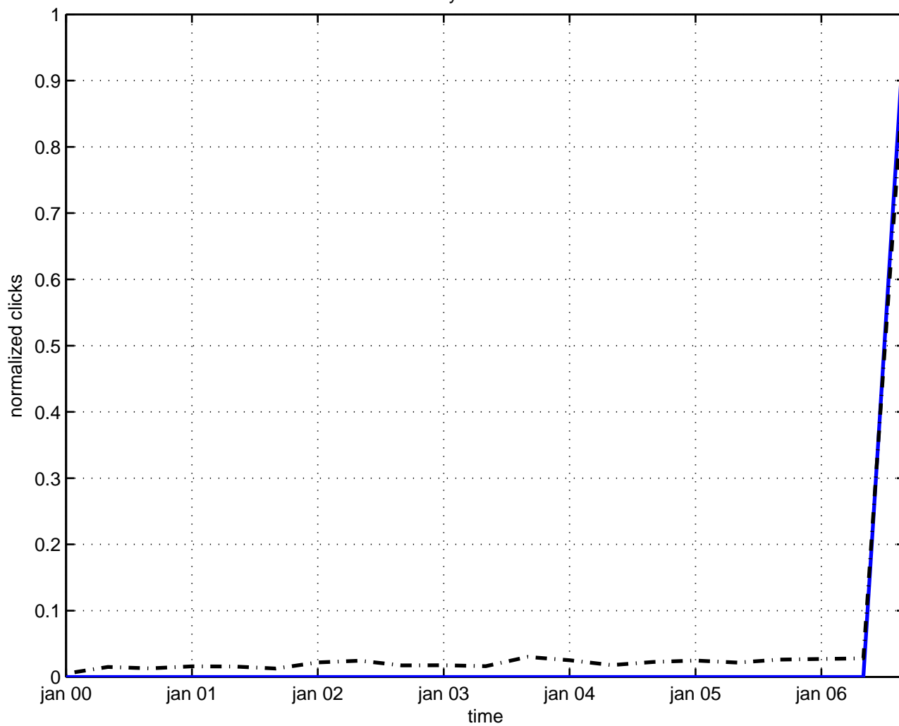
isometry transformation
