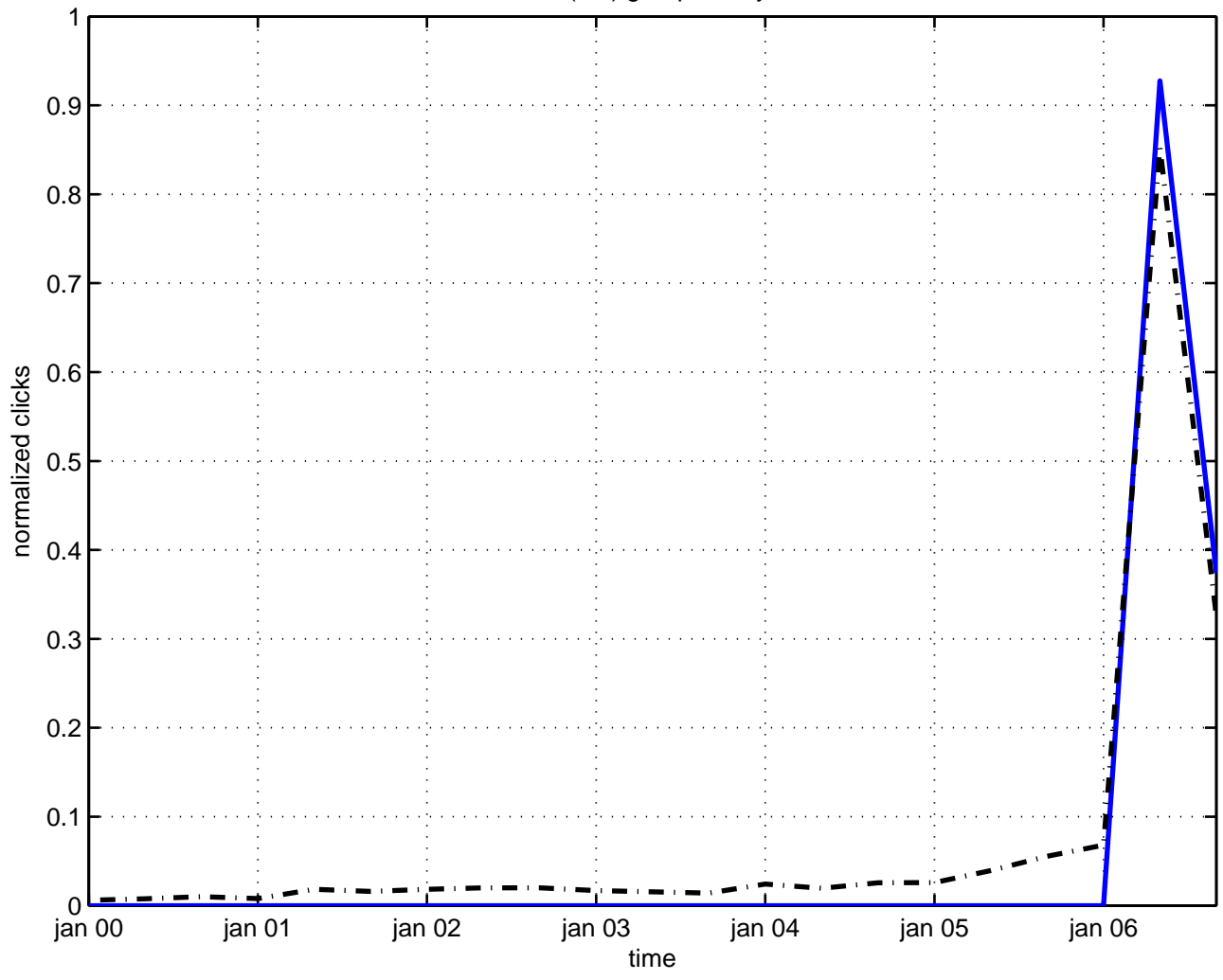
iso(n,1) group theory
