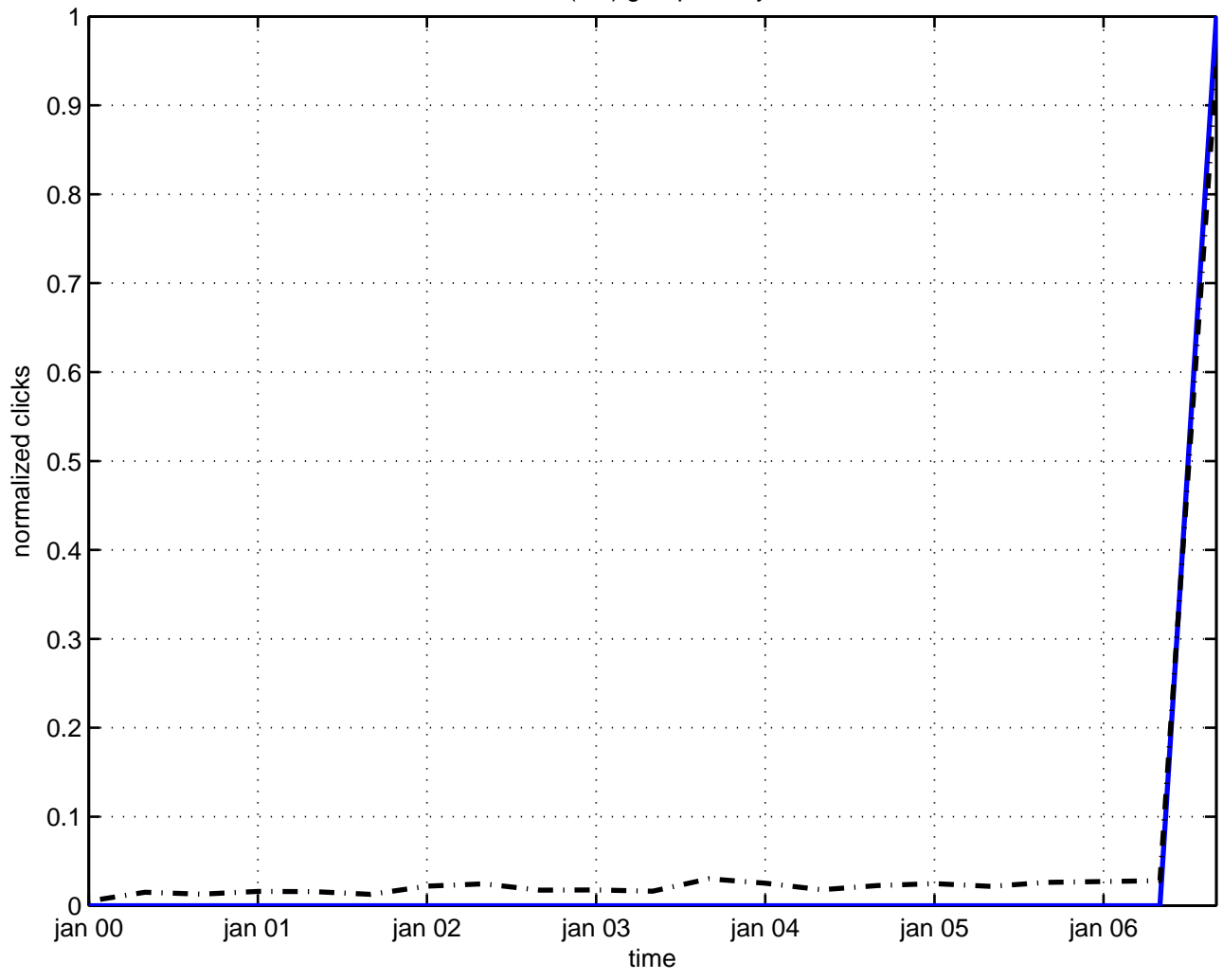
iso(2,3) group theory
