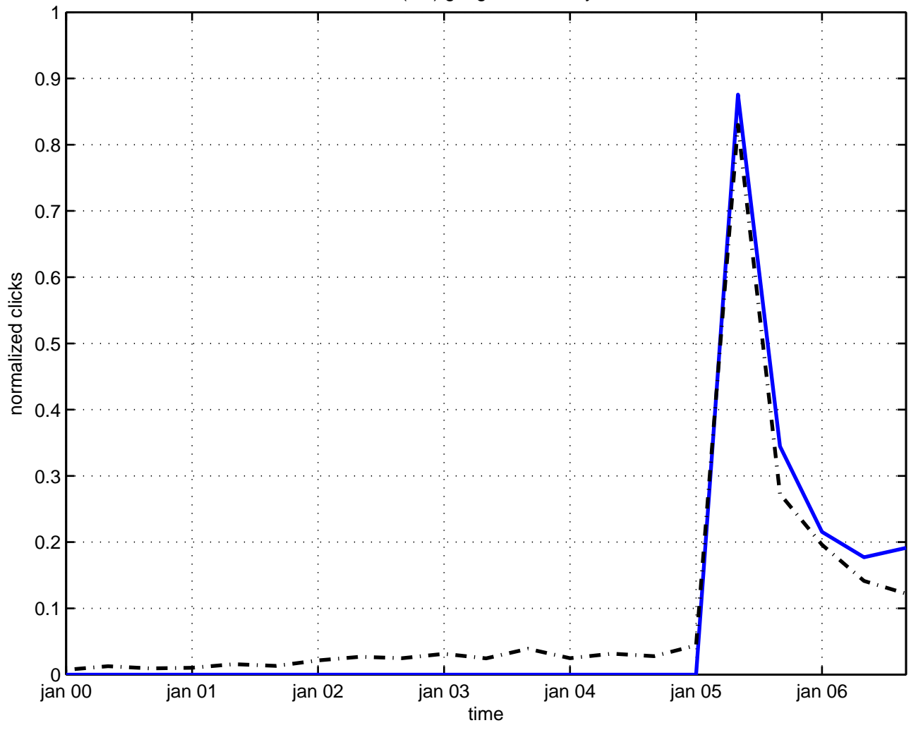
iso(2,1) gauge field theory
