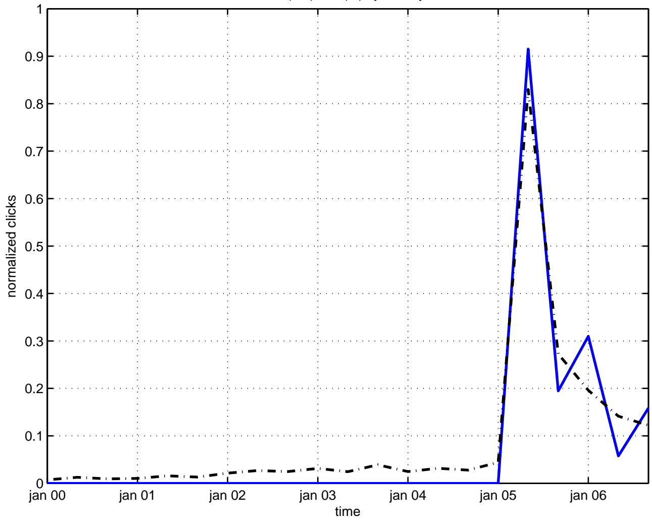
iso(1,n) x so(m) symmetry
