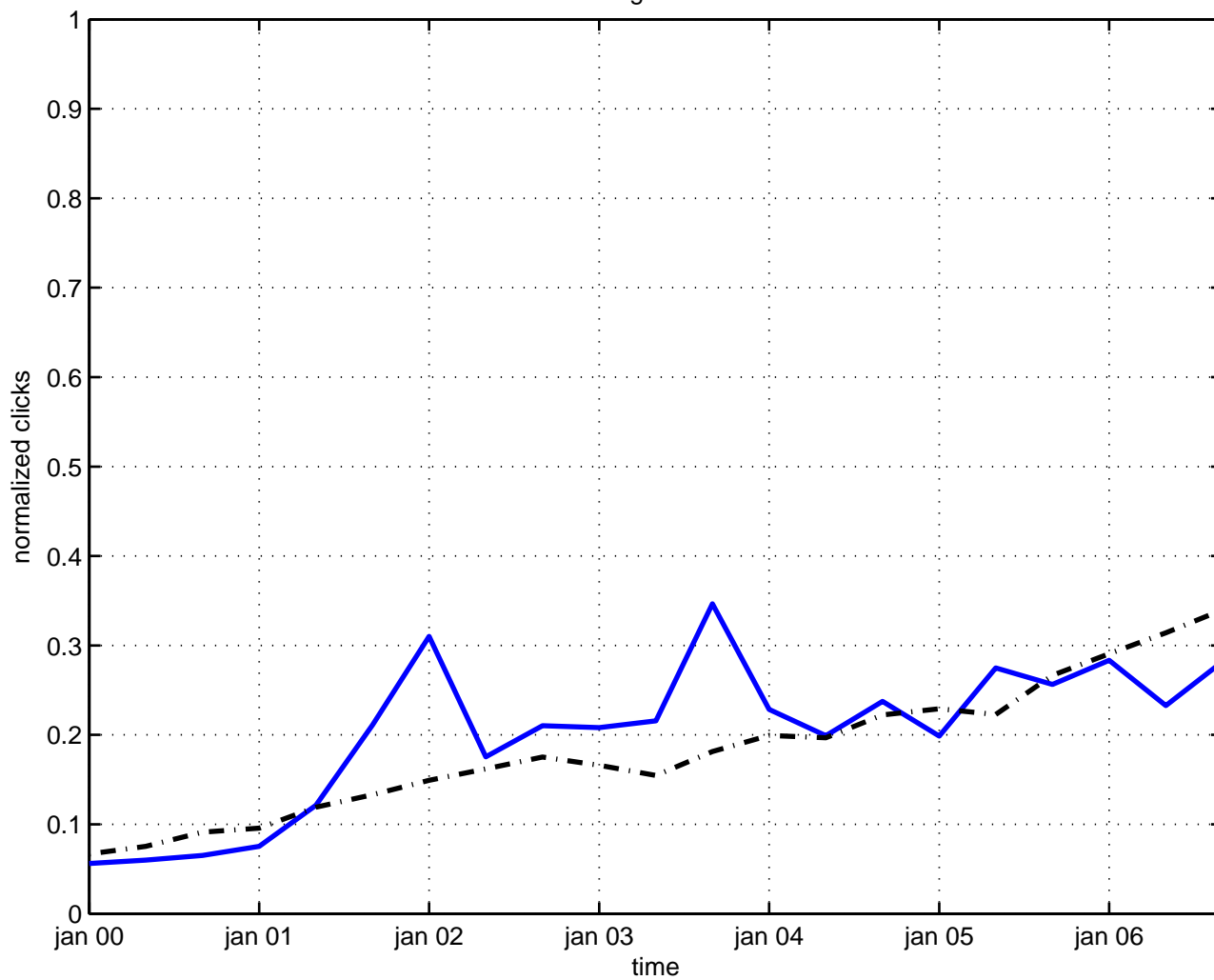
ising model
