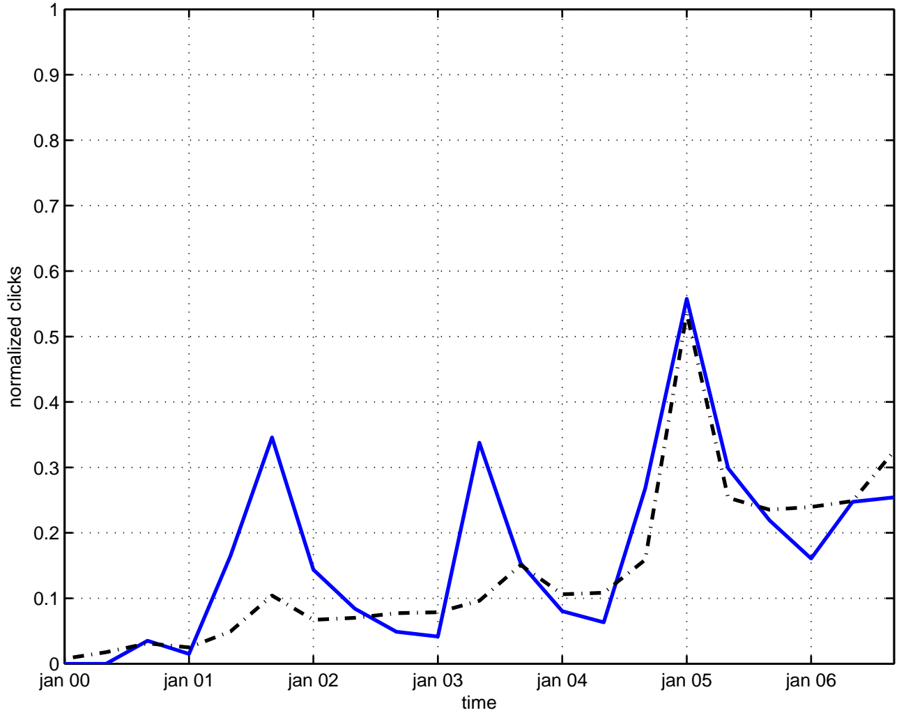
invariance scaling
