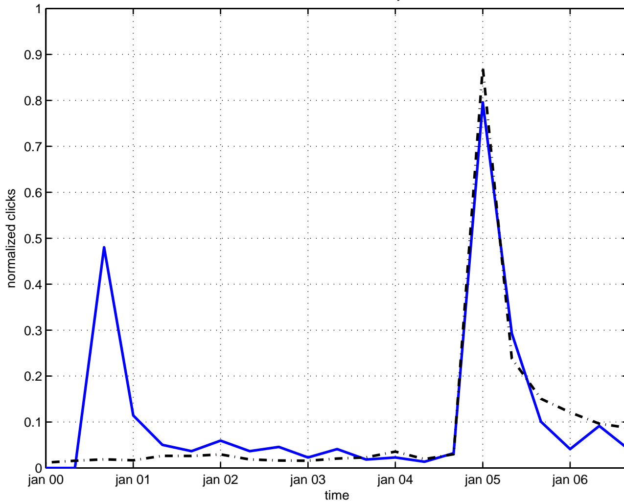
invariance monodromy
