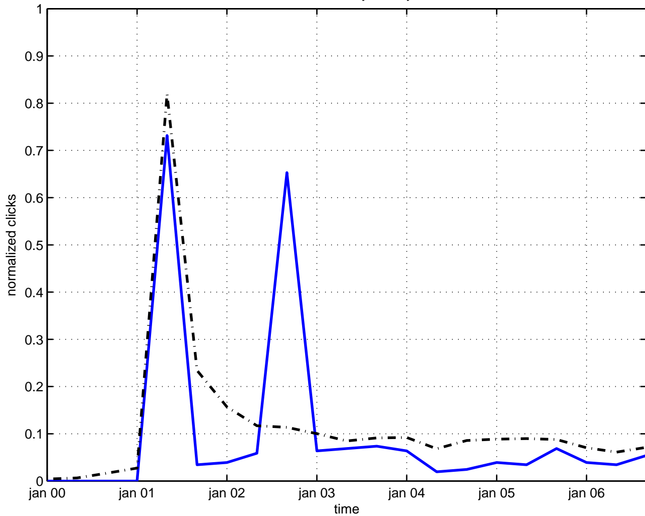
interference symmetry
