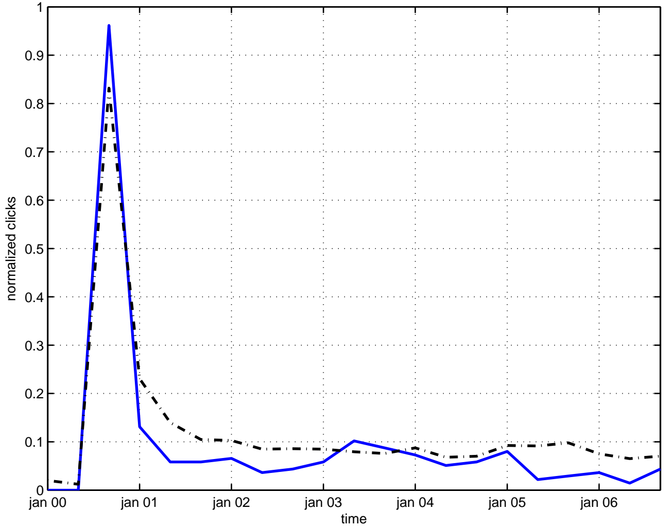
interference quark
