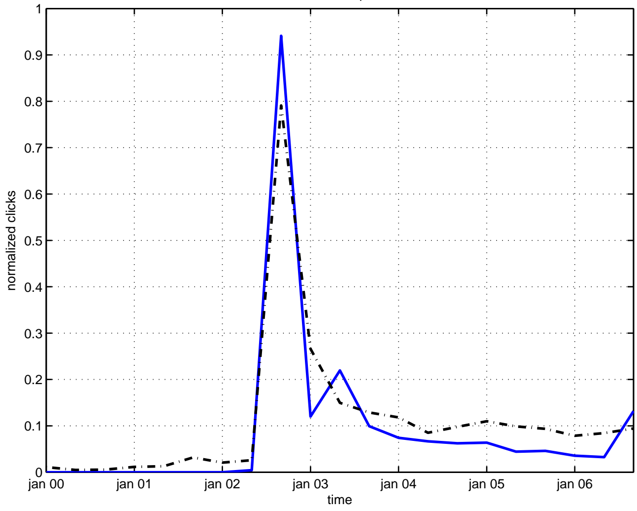
interference operator
