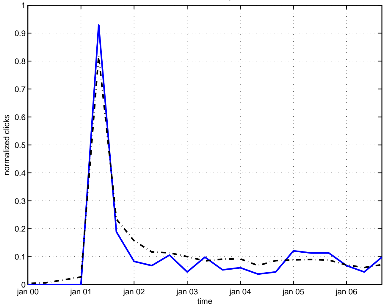
interference multiplet
