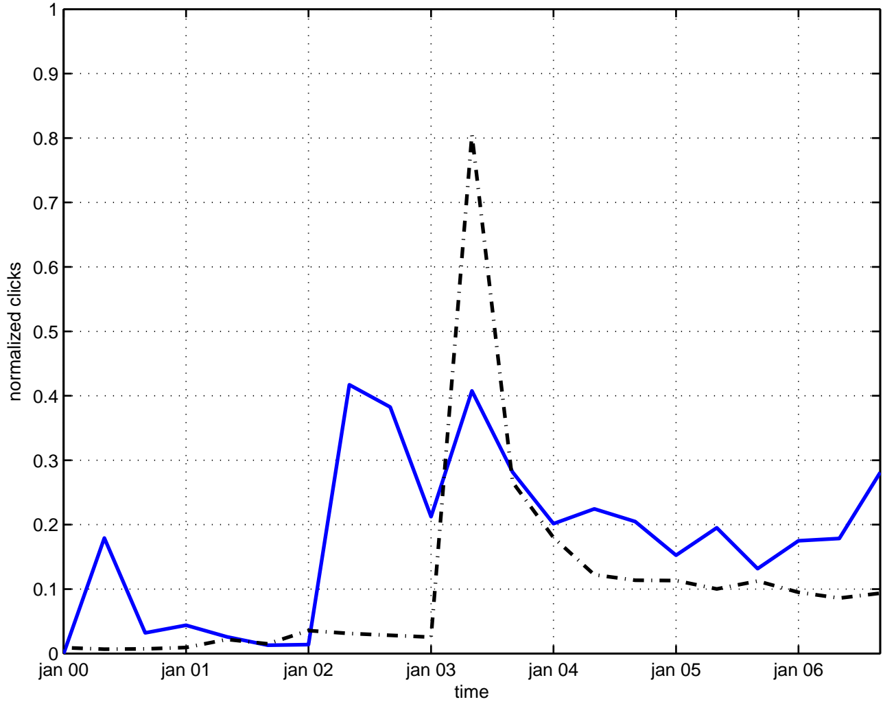
interaction string
